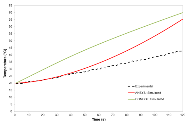
b) Comparison between FBG data and simulation results
