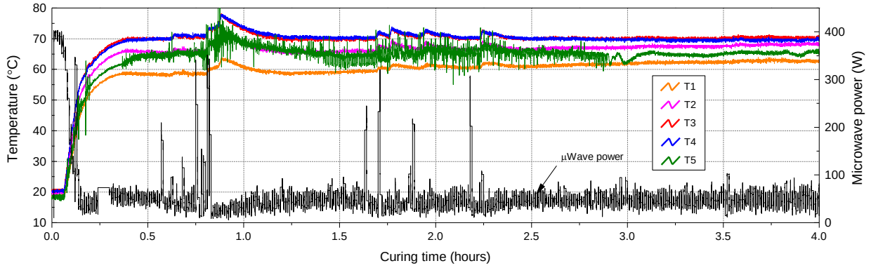
Fig. 5 Temperature feedback control of concrete cube cured for 4hrs (max internal temperature of 70°C)
