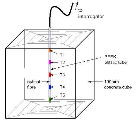
Fig. 3 FBG probe layout
