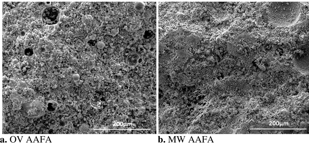
Fig. 7. SEM images of AAFA samples
