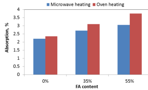
Figure 4 Water absorption at 7 days
