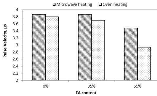
Figure 6 Ultrasonic pulse velocity at 7 days
