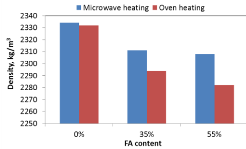
Figure 3 Density at 7 days
