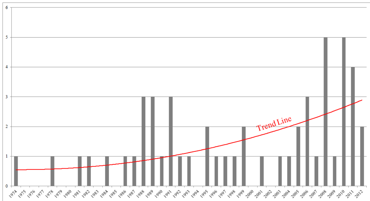
Figure 1: Number of reviews published per year
