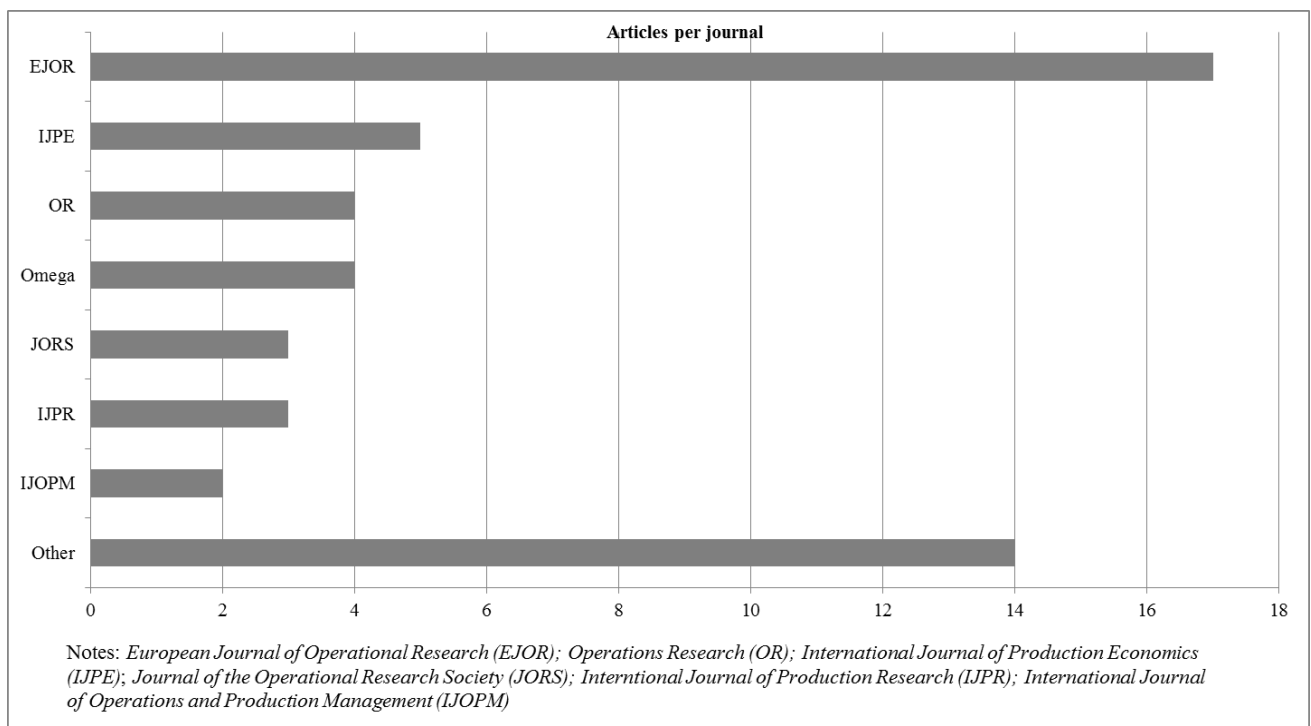
Figure 2: Number of reviews published per journal
