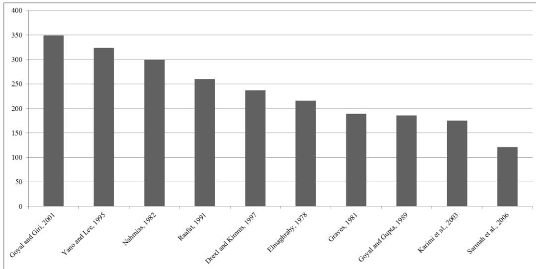
Figure 3: Most frequently cited literature reviews in lot sizing
