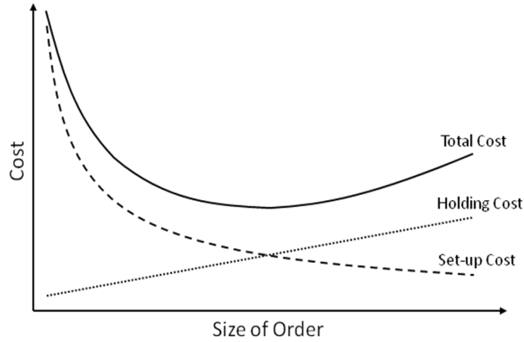
Figure 4: Relevant cost curves for Harris' lot size model
