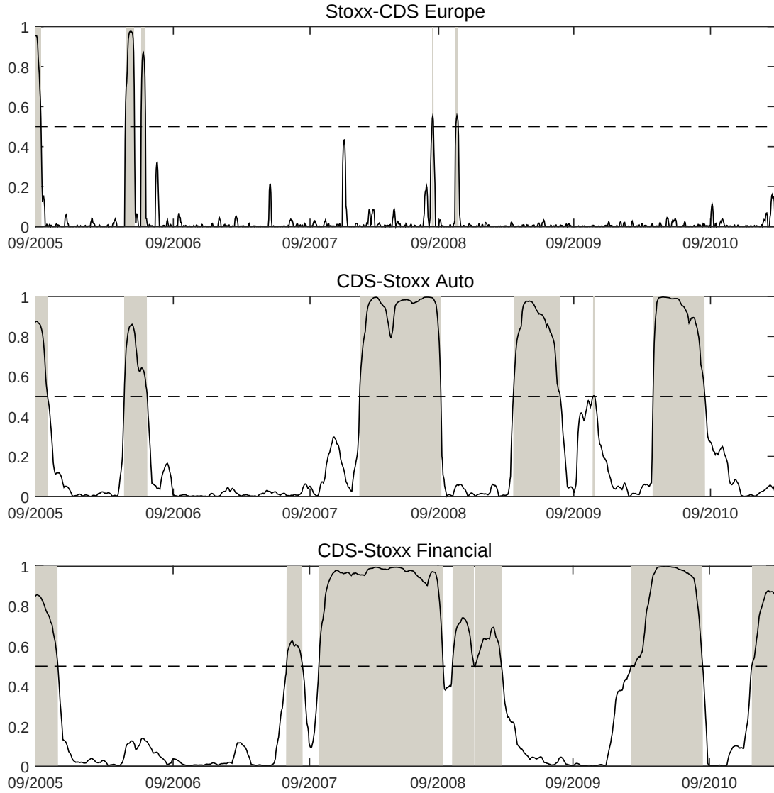
Figure 2: Smoothed Probability of High Dependence Regime: The graphs show the smoothed probability of high dependence regime inferred from the RS-ARMA Student's t copula model for pairs of CDS-equity indices. Days when the smoothed probability exceeds 0.5 (fall below 0.5) are shaded in grey (white) to indicate that they pertain to the high or 'crisis' (low or 'normal') dependence regime according to the model.
