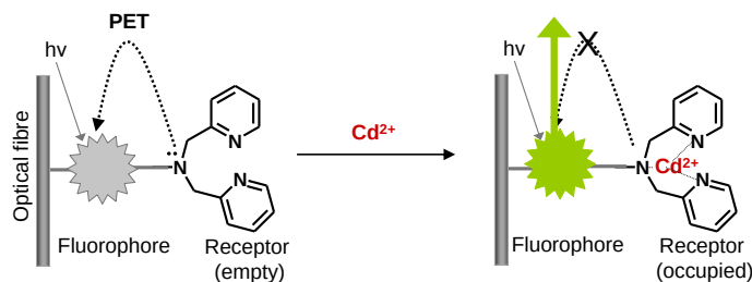
Fig. 1. Illustration of fluorescence switching on by \text{Cd}^{2+} binding via a PET mechanism.
