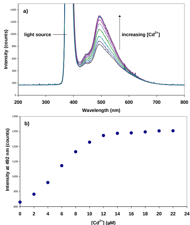
Fig. 4. a) Fluorescence spectra of the sensor probe in deionised water with the addition of Cd 2+ b) Corresponding plot showing the change of fluorescence intensity with changing Cd 2+ concentration.
