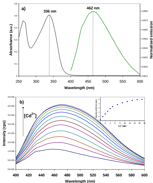
Fig. 2. a) Absorption and emission spectra of CDA (20 μM) in H 2 O/MeCN (7:3, v/v). Emission spectrum recorded with \lambda_{\text{ex}} = 336 nm. b) Emission spectra of CDA at [Cd 2+ ] ranging from 0 to 17 μM. The inset shows the titration plots at 462 nm ( \lambda_{\text{ex}} = 336 nm).
