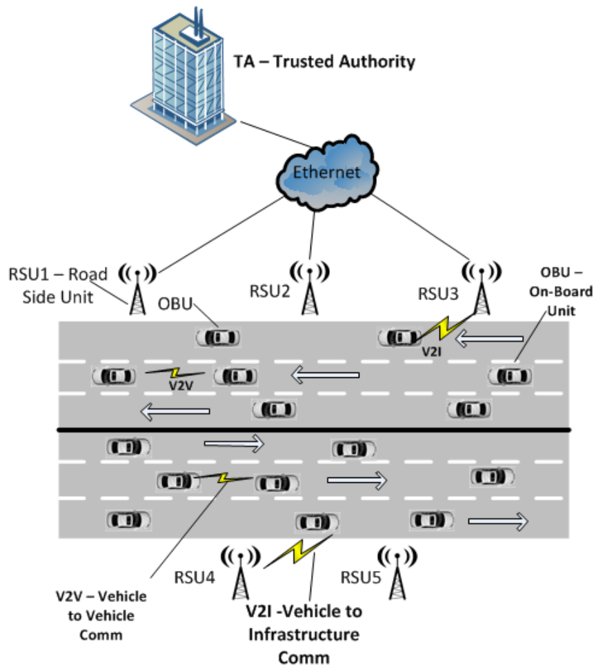
Figure 2-1: VANET Architecture
