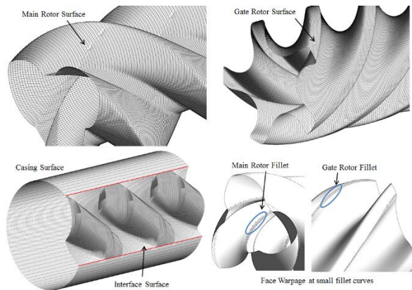
Figure 15 Surface mesh on the rotor, casing and the rack interface
