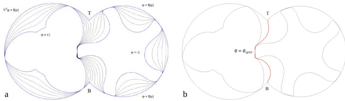
Figure 4 Solution of Laplace equation – a) Iso-potential lines and b) Splitting curve
