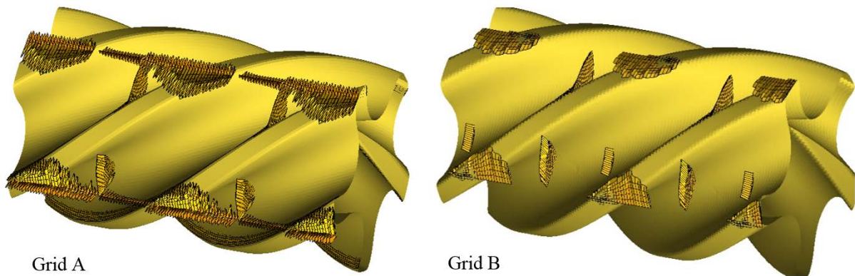
Figure 19 Comparison of cells with Equiangular Skewness factor &lt; 0.15
