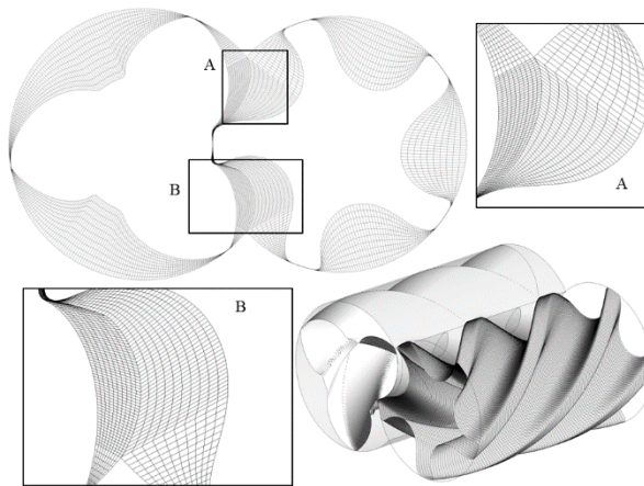
Figure 14 Grid generated with background blocking in screw compressor rotor
