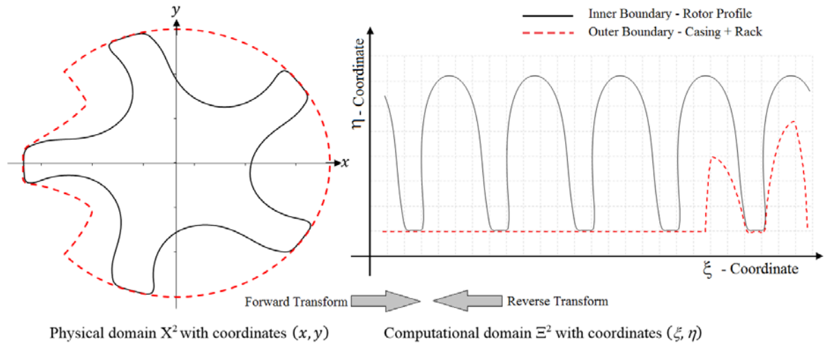
Figure 7 Physical and Computational domains with coordinate transformation of inner and outer boundary
