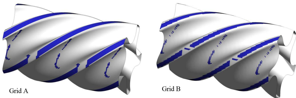
Figure 20 Comparison of regions with aspect ratio > 200
