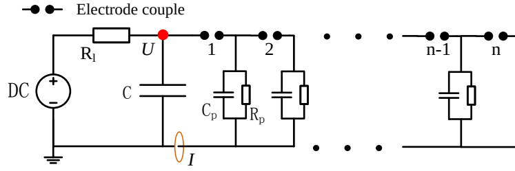
Fig. 1 The multichannel discharge circuit schematic diagram
