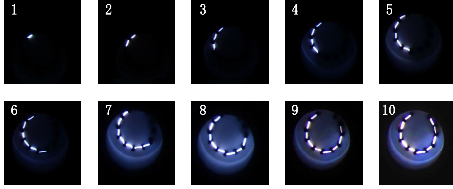
Fig. 7 The discharge images of different channels of the ME-PSJA
