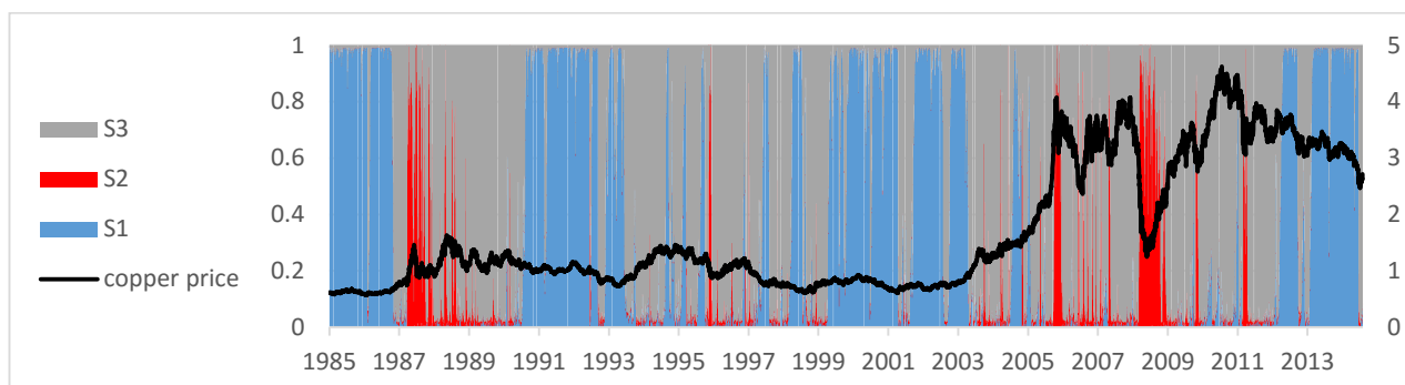
Figure 3: States transitions real probabilities
