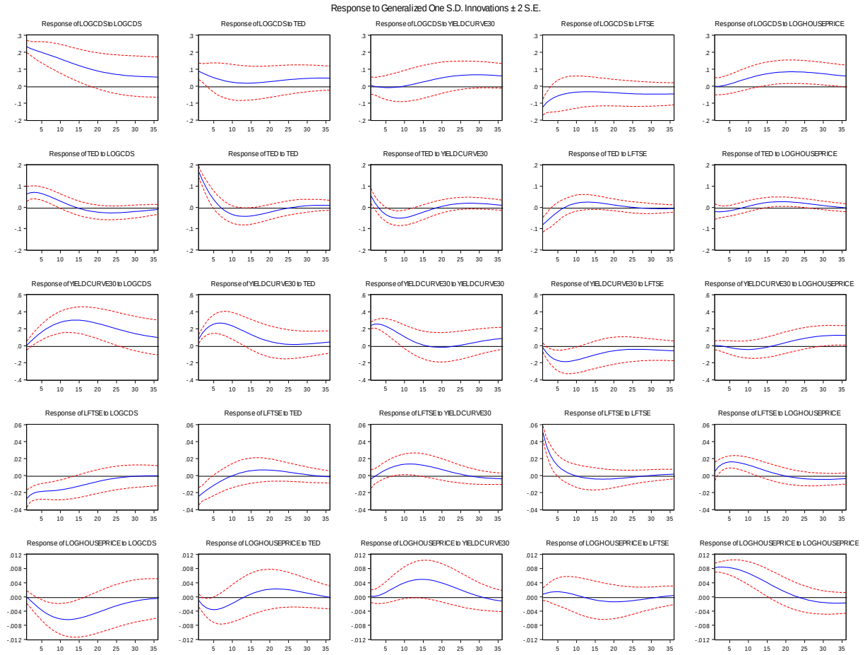
Figure 7: Generalised impulse responses with change in ordering for robustness
