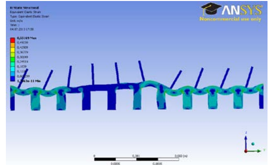
Figure 8: FEM-results of membrane and corresponding flap deflections for establishing a metachronal wave.
