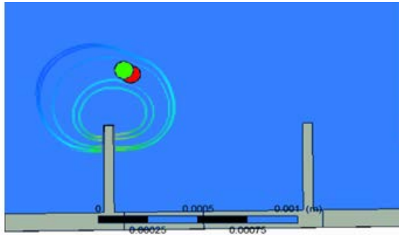
Figure 7: Displacement of a particle (100 \mu\text{m} in diameter) after two membrane bending cycles. The left green particle corresponds to the start position and the right red particle to the end position after two complete load cycles. The distance between the two positions is about 40 \mu\text{m} . The colored lines are streamlines of a specific time step.
