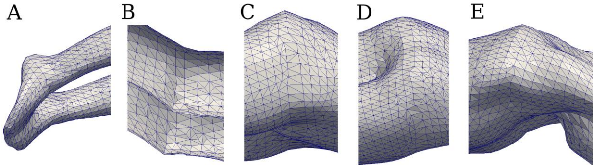
Figure 12: Surface repairing. Corrected surface deformation irregularities from figure 11 when applying the skin-stretching method in rigid human swimming at A) the feet, B) the knees C & D) and the hips and E) the shoulders.
