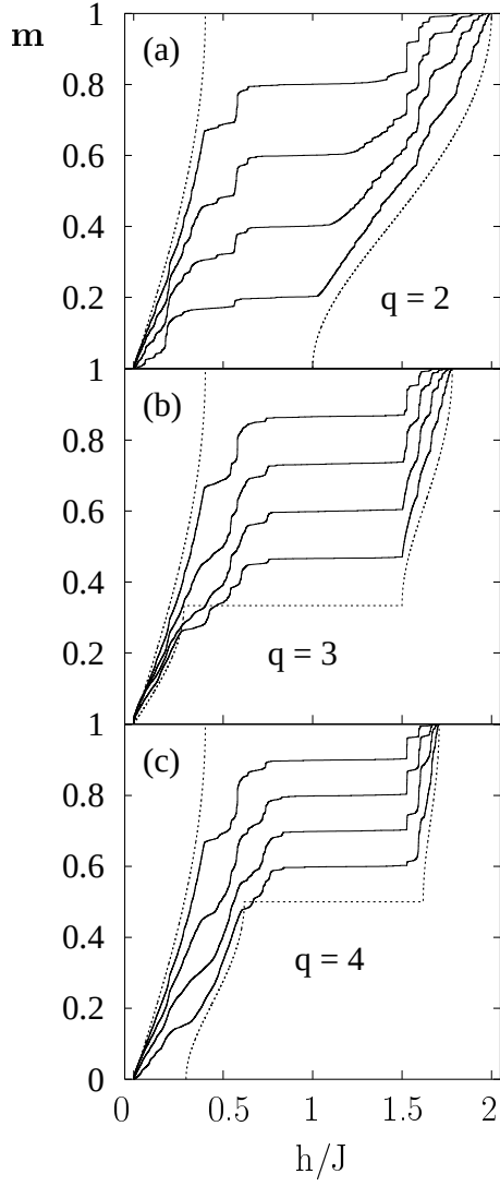
FIG. 1. Magnetization curves of modulated XX spin chains with q = 2 (a), 3 (b) and 4 (c), immersed in disordered binary backgrounds of strength p . Solid lines represent averages over 100 samples with 5 \times 10^4 sites, J'/J_0 = 0.2 , \gamma J = 0.5 and p = 0.2, 0.4, 0.6, 0.8 in ascending order. The left and rightmost dotted lines denote respectively the pure uniform and pure modulated cases p = 1 and p = 0 .
