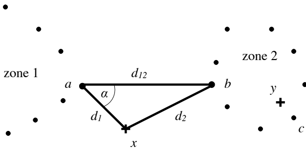
Figure 1. Distances of point x to closest points of two zones.
