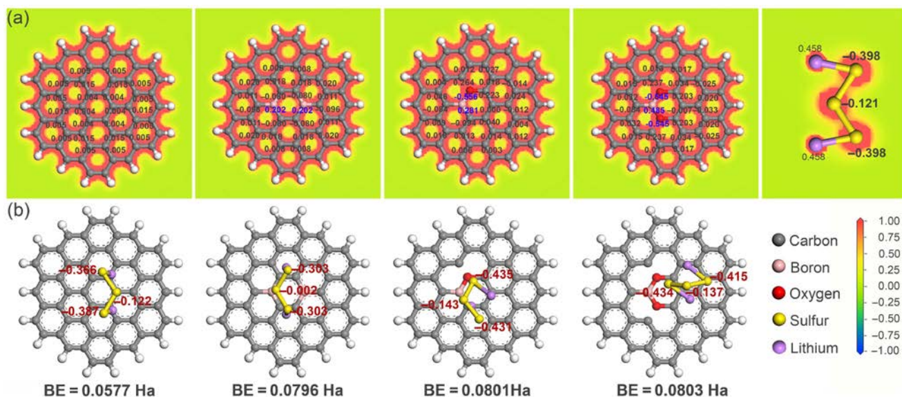
Figure 5 (a) Optimized geometries of the boron-doped and undoped carbon layers and \text{Li}_2\text{S}_3 molecule and the isosurfaces of the cross-sectional density difference. (b) Top views of \text{Li}_2\text{S}_3 molecule adsorbed on the boron-doped and boron-undoped carbon surface, and the corresponding binding energy values. The optimized atomic charges of specific atoms are also provided here, and the charge distribution on each atom is evaluated using the Mulliken population analysis.
