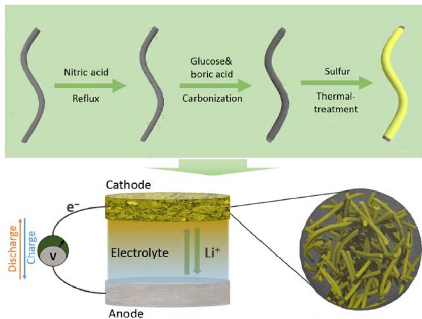
Scheme 1 Schematic illustration of the synthetic route to BMC.
