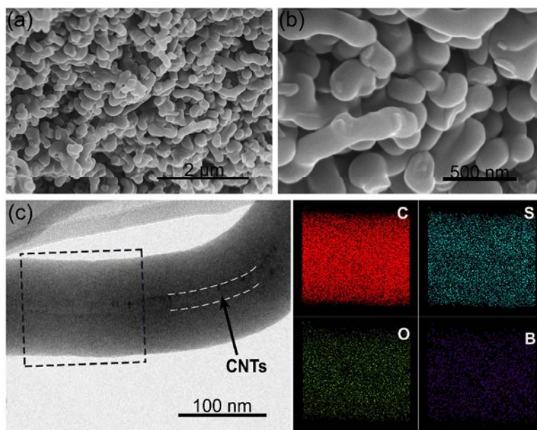
Figure 2 (a) and (b) SEM images of BMC/LS composite. (c) TEM image of the BMC/LS composite and the corresponding EDX elemental maps of the region marked with a black rectangle.
