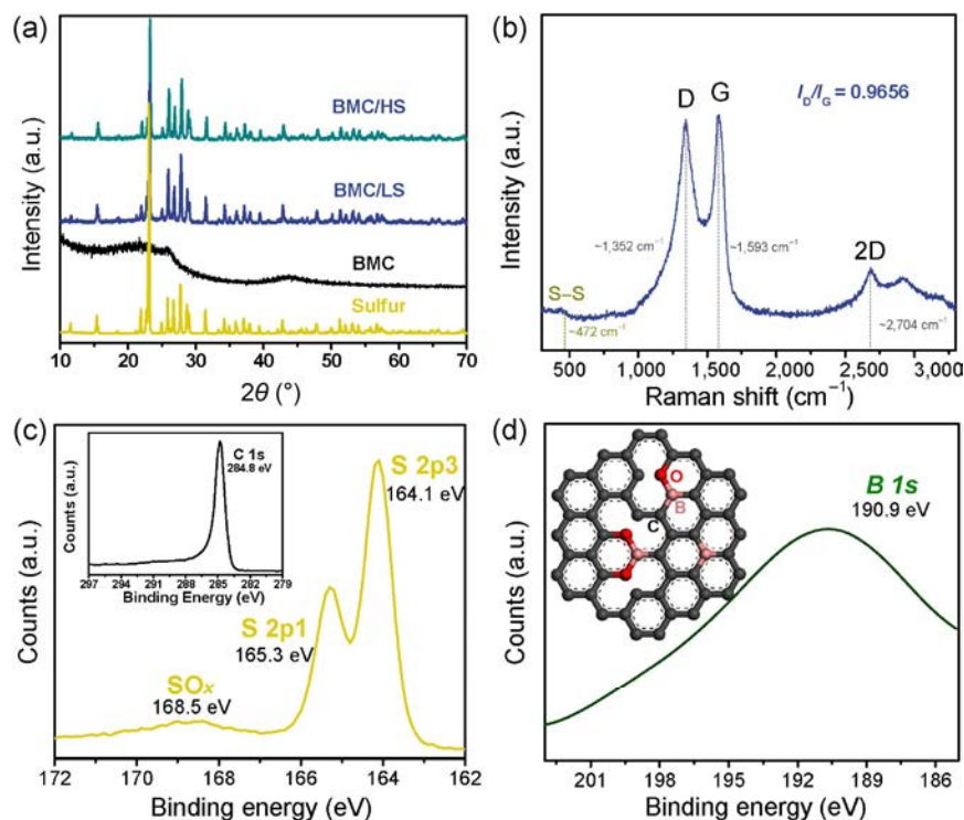
Figure 3 (a) XRD patterns of sulfur, BMC, BMC/LS and BMC/HS. (b) Raman spectrum of the BMC/LS composite and XPS spectra of (c) S 2p regions and (d) B 1s region of the BMC/LS composite. The inset in (c) represents the C 1s region.
