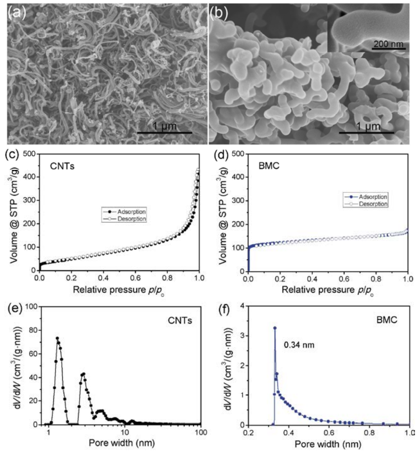
Figure 1 SEM images of (a) CNTs and (b) BMC, and the corresponding nitrogen sorption isotherms for (c) CNTs and (d) BMC; (e) the pore size distribution determined for CNTs using NLDFT method and (f) the pore size distribution determined for BMC using H-K method.
