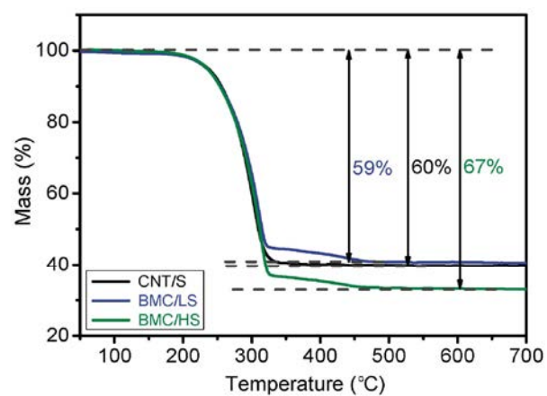
Figure S2 TGA curves of the CNT/S, BMC/LS and BMC/HS composites recorded in Ar at a heating rate of 10 °C/min.
