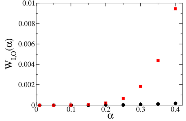
FIG. 4. Cumulative weight W_\lambda vs \alpha , see Eq. (35), of the negative energy states in the variational wave function for Z = 1 , where \lambda = I ( \lambda = O ) corresponds to black circles (red squares).
