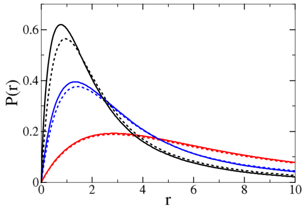
FIG. 5. Radial density P(r) vs distance r from the impurity (in units of \hbar v_F / \Delta ) of the spin-singlet two-body bound state, cf. Eq. (47), for Z = 1 and several values of \alpha . The solid lines correspond to the relativistic case for \alpha = 0.1, 0.2 , and 0.3 , shown in red, blue, and black colors (from bottom to top), respectively. The dashed lines indicate the corresponding nonrelativistic results.
