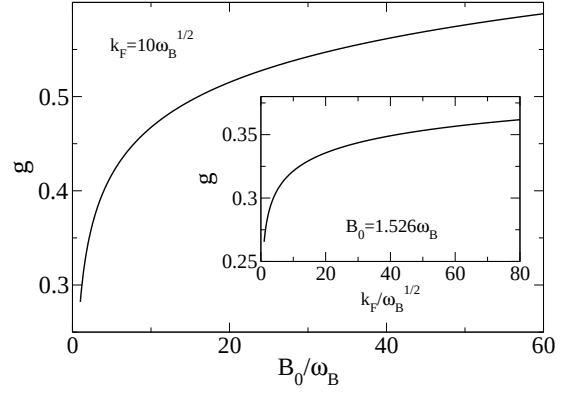
FIG. 5: TLL parameter g in Eq. (32) for \alpha = 1 and D = 100/\sqrt{\omega_B} . Main panel: g as a function of B_0/\omega_B for k_F = 10\sqrt{\omega_B} . Inset: g vs k_F/\sqrt{\omega_B} for B_0 = 1.526\omega_B . Note that the regime \lambda \ll d translates into k_F \gg \frac{18}{\sqrt{3}}\omega_B^2 B_0^{-5/2} , which here implies k_F/\sqrt{\omega_B} > 1 .
