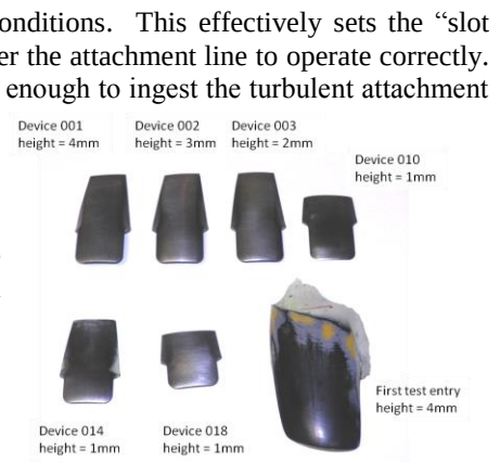
Figure 6 Gaster Slot devices tested
