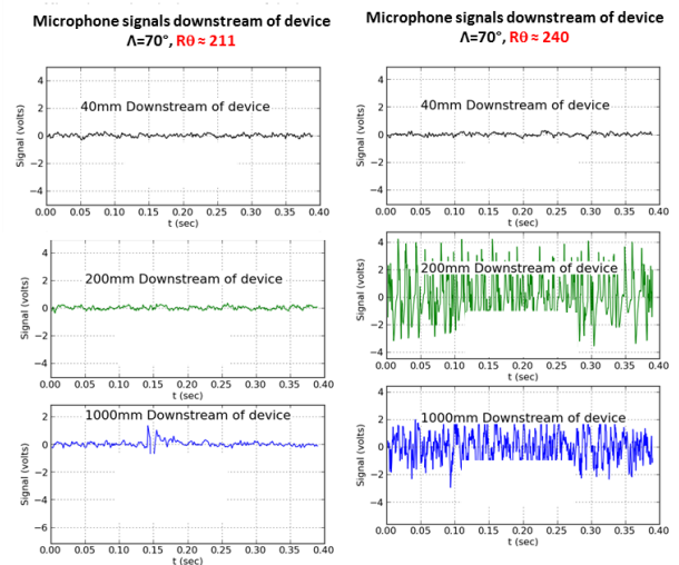
Figure 9 Microphone signals at high R\theta
