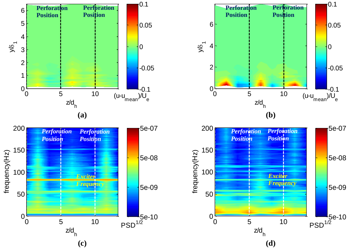
Figure 8. Stationary wave plots, indicating the presence of vortex structures: (a) shows case with disconnected pump and perforated insert panel; (b) with a connected pump, v_A/U_e = 0.6595 \times 10^{-3} of suction, and a perforated insert panel; (c) shows spectral energy distribution for the case with no pump, (d) shows it for the case with a pump. U_e was set to 8m/s, d_h was 0.6mm, f_k = 81\text{Hz} , and x was located at x/C = 0.3193 for both of these cases.
