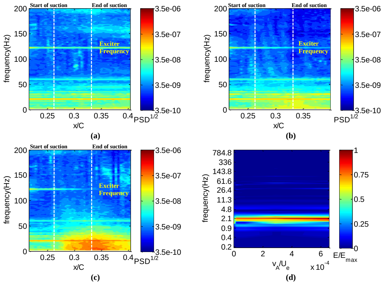
Figure 3. Power Spectral Density plots of Hot-wire and microphone sensors at z=0 mm, U_e=18 m/s, d_h=0.6 mm, and f_k=121 Hz: (a) shows no suction with perforations covered, (b) shows v_A/U_e=0.0824 E-3, (c) shows v_A/U_e=0.2886 E-3 of suction, (d) shows microphone energy for different suction rates.
