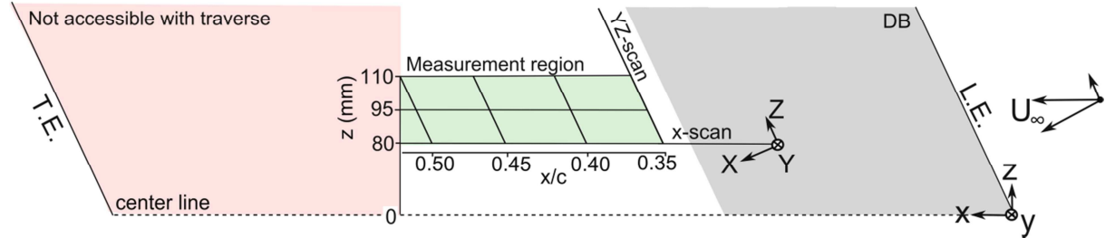
Figure 6: Coordinate systems used in measurements together with the hot wire scans which are carried out.
