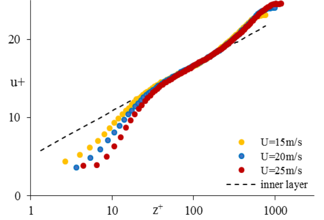
Fig. 3: Velocity profiles along unperforated plate at x=730\text{mm} . The inner layer is defined by z^+ = 2.5 \ln u^+ + 5.1 .
