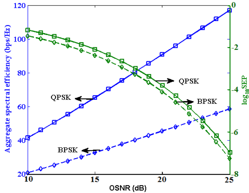
Fig. 8. Aggregate spectral efficiency and SEP as a function of OSNR for BPSK ( \alpha = \infty ) and QPSK ( \alpha = 1 ) modulated MCF OI transmission.
