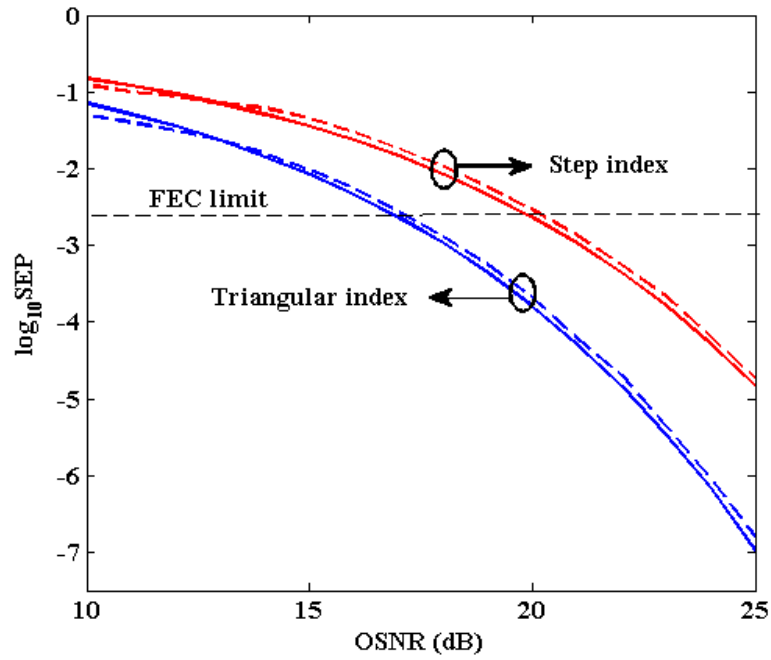
Fig. 4. SEP as a function of OSNR for QPSK system in step index and triangular index MCF OI. Solid curves are obtained from theory of Section 2 and dashed curves from simulation experiment of Section 3.
