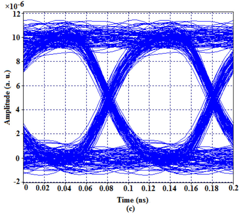
Figs. 7. Eye diagrams of (a) BPSK and (b) QPSK signal for step index MCF and (c) Eye diagram of QPSK signal for triangular index MCF.
