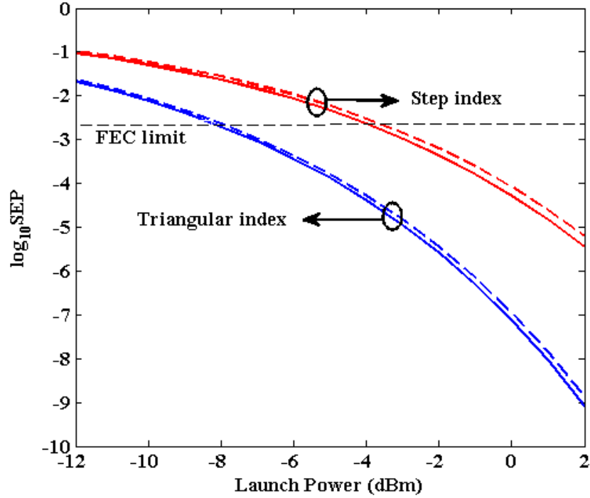
Fig. 5. SEP as a function of launch power for QPSK modulated system in step index and triangular index MCF OI.
