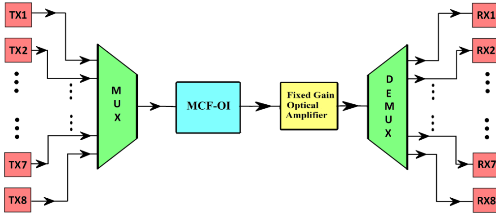
Fig. 3(a) Simulation setup for QPSK modulated short reach transmission system using 8-core MCF. TX: transmitter, RX: receiver, MUX: multiplexer, DEMUX: demultiplexer.
