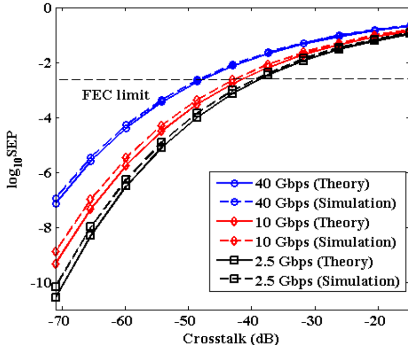
Fig. 6. SEP as a function of inter-core crosstalk for various QPSK modulated Signal.
