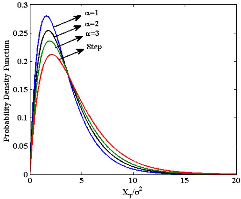
Fig. 2. Crosstalk distributions for different index profile \alpha in 8-core MCF.
