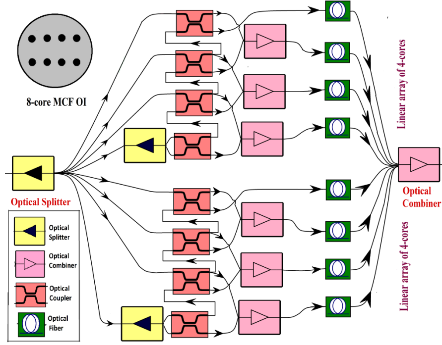
Fig. 3(b). Equivalent simulation model of 8-core MCF OI. The schematic of rectangular array 8-core MCF with triangular index profile is shown in inset [8, 9].
