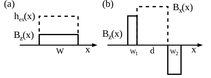
FIG. 1: Profiles of magnetic field and exchange field considered in this paper. In case (b) the exchange field is included in B_x .
