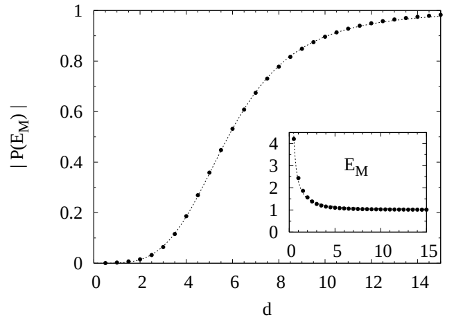
FIG. 6: Maximum of the total polarization |P(E_M)| as a function of d for the same structure and parameters as in Fig. 5. In the inset: plot of the energy E_M where the peak of |P(E)| is located as function of d .
