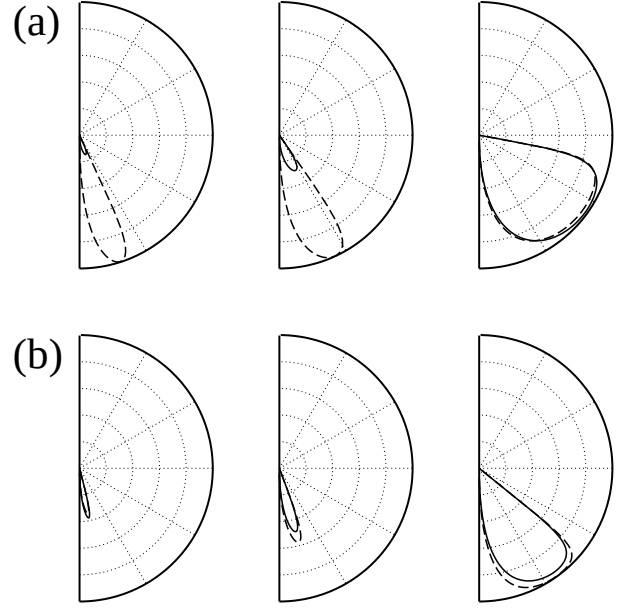
FIG. 2: (a) Angular plot of the transmission through a rectangular magnetic barrier of width W = 2 (in units of \ell_B ) with \lambda = 0.2 for spin-up (solid lines) and spin-down (dashed lines) quasiparticles at energy E = 1.05, 1.1, 1.7 (from left to right, in units of E_m ); (b) the same for a barrier of width W = 6 at energy E = 3.05, 3.1, 3.7 . Here we set B = 1 T, so that E_m \approx 25 meV and an energy increment of 0.1 corresponds to 2.5 meV.
