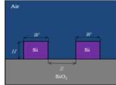
Fig . 2. Cross-section of two identical coupled NWs.
