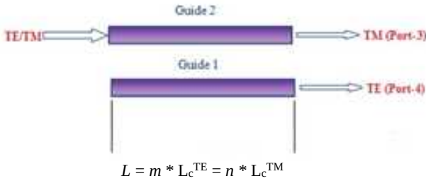
Fig . 1. Principle of a polarization splitter.
