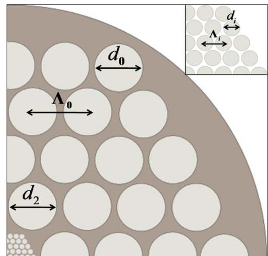
Fig.1. Cross-section of porous core PCF, N_{\text{core}} = 4 and N_{\text{clad}} = 4 . Air holes are arranged in the cladding with \Lambda_0 = outer pitch, d_0 = outer diameter. Inset shows \Lambda_1 = inner pitch, d_1 = inner diameter in the porous core.
