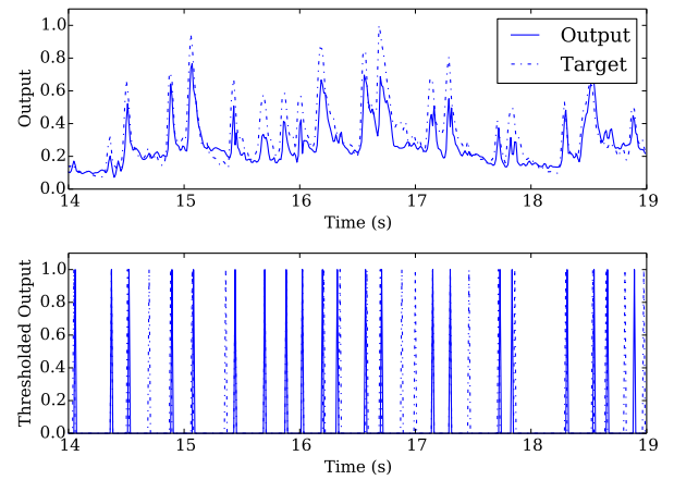
Figure 6. The output of the GFNN-LSTM. The top figure shown the predicted onset likelihood, the bottom figure displays the threshold events.
