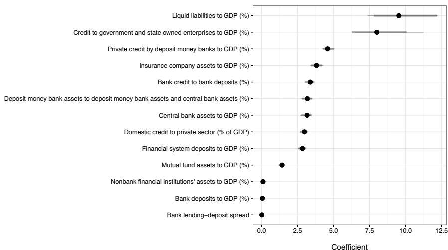
Figure A-6: Estimated Item Discrimination Parameters
