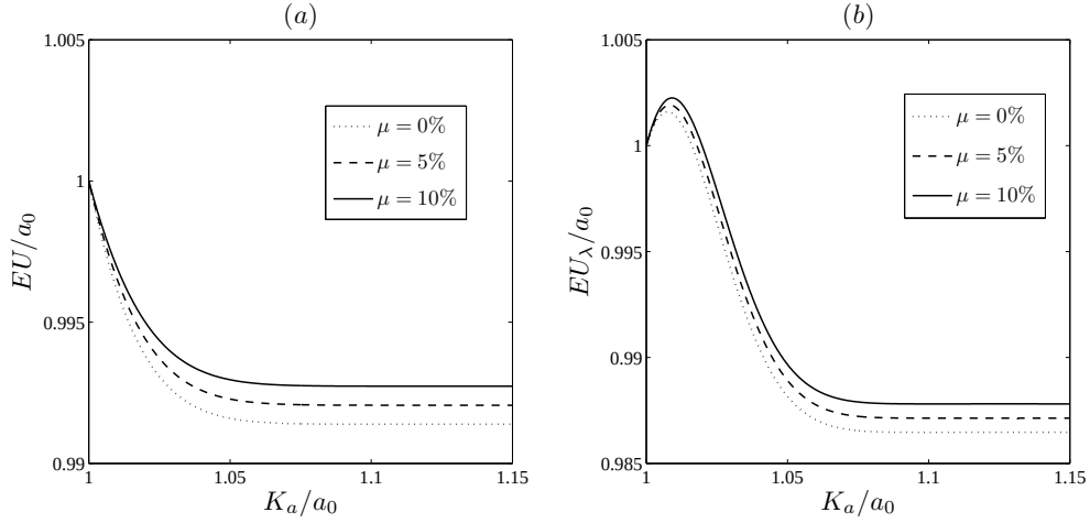
Figure 4: The expected utility of a sell limit order strategy for a risk-averse trader ( \varphi = 0.01 ) as a function of the limit price: (a) no delay in execution ( a_0 = b_0 = 1000 ), (b) in presence of a random delay in limit order execution ( a_0 = 1000, b_0 = 995 ). Results are shown for parameters in Table II.
