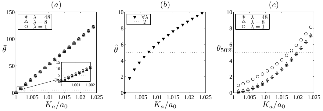
Figure 2: The characteristics of the most common time-to-fill of sell limit orders submitted at different prices K_a \geq a_0 : (a) the average time-to-fill, (b) the mode time-to-fill, (c) the median time-to-fill. Results are shown for parameters in Table II.
