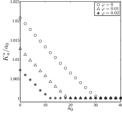
Figure 6: The optimal limit sell price for a risk-averse trader as a function of initial spread s_0 . Results are shown for parameters in Table II .
