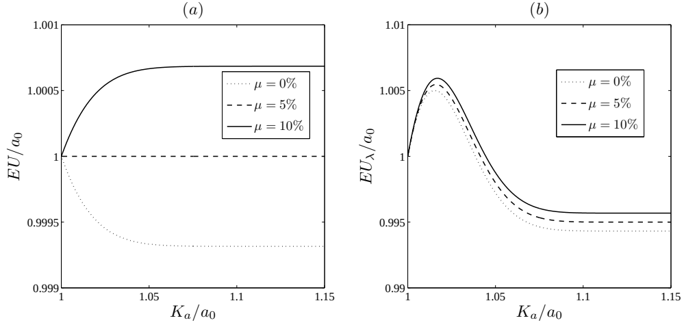
Figure 3: The expected utility of a sell limit order strategy for a risk-neutral trader ( \varphi = 0 ) as a function of the limit price: (a) no delay in execution ( a_0 = b_0 = 1000 ), (b) in presence of a random delay in limit order execution ( a_0 = 1000, b_0 = 995 ). Results are shown for parameters in Table II.
