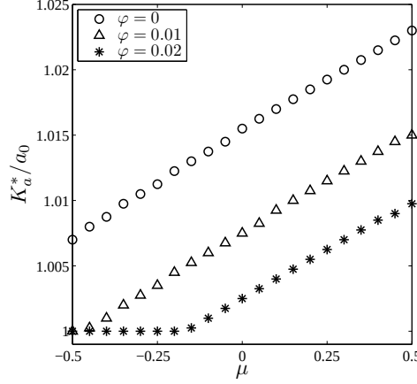
Figure 5: The optimal limit sell price for a risk-averse trader as a function of the price drift in presence of a random delay in limit order execution. Results are shown for parameters in Table II.
