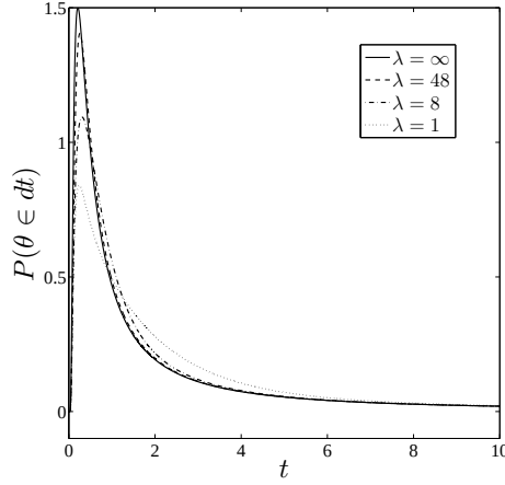
Figure 1: The probability density function of the time-to-fill of a limit order. Results are shown for parameters in Table II and K_a/a_0 = 1.01 .
