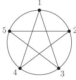
Figure 1. The pentacle diagram representing the CHY-integrand defined by the two-cycles \{(1,2,3,4,5), (1,3,5,2,4)\} .
