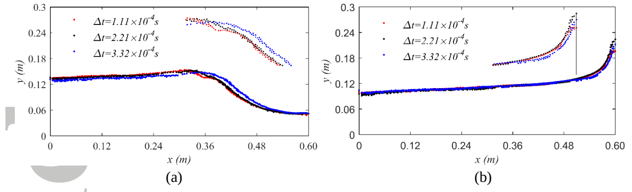
Figure 16: Snapshots of interfaces obtained using the time steps of 1.11 \times 10^{-4} \text{ s} , 2.21 \times 10^{-4} \text{ s} and 3.32 \times 10^{-4} \text{ s} at t = 1.43 \text{ s} (a) and t = 1.56 \text{ s} (b).
