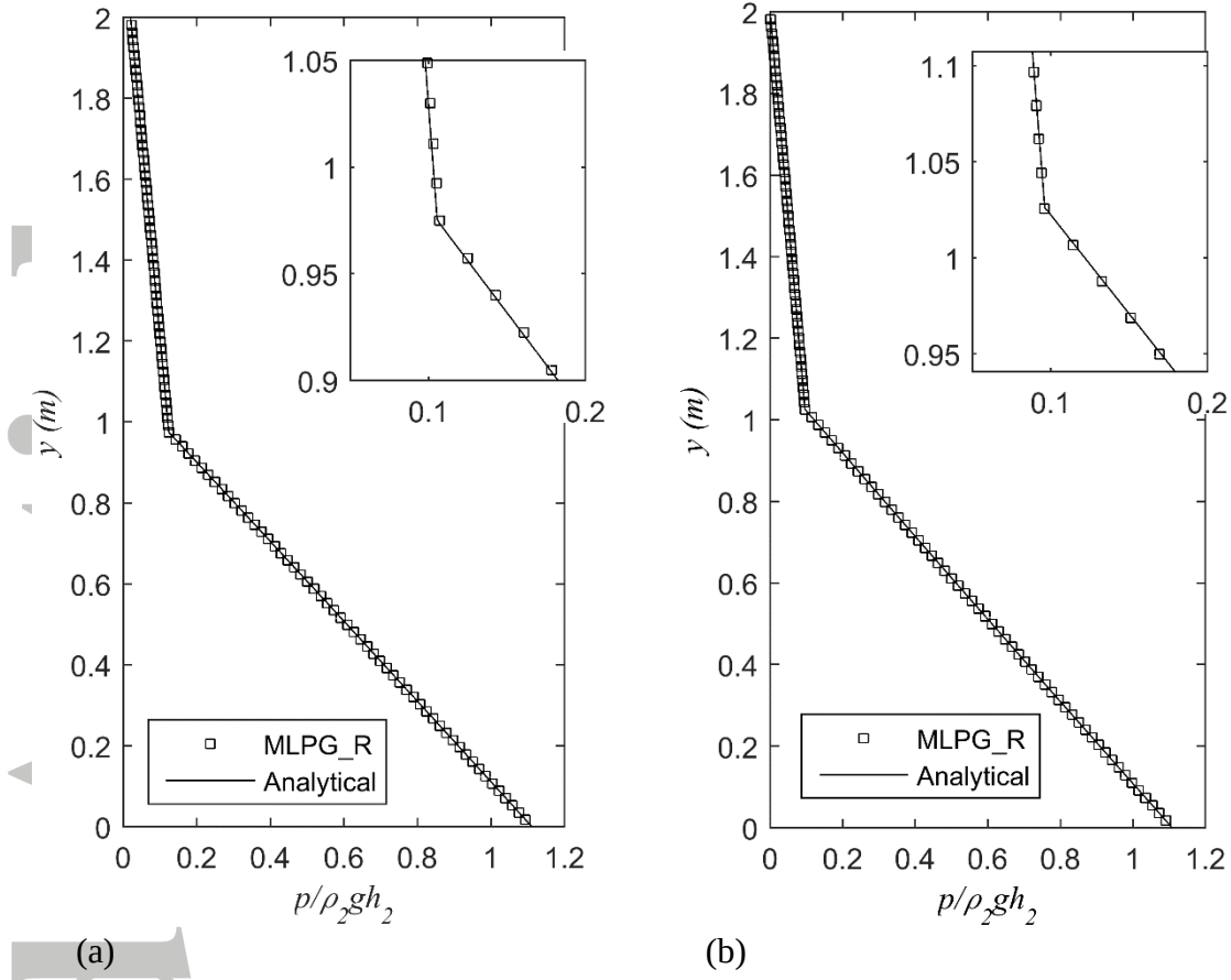
Figure 13: Pressure distributions along the depth at x=0.3\text{m} (a) and x=1.7\text{m} (b) at t\sqrt{g/h_2} = 1.4 for the case with density ratio of 10. The inset the results near the interface. The analytical solution is from [41].
