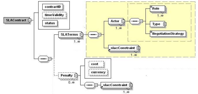
Figure 3. High Level Schema for SLA Specification
