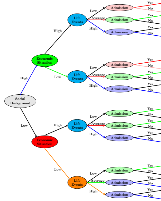
FIG 1. MAP CEG for the CHDS data under the restriction of the node ordering S \prec E \prec L \prec H , presented as an event tree.
