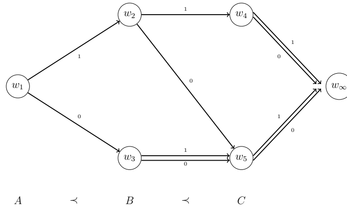
FIG 6. SCEG corresponding to the stages partition (iv) in Table 1. Node w_1 corresponds to the stage partition (A), node w_2 to the stage ( B_1 ) and w_3 to ( B_0 ). Node w_4 corresponds to the stage partition ( C_{11} ), and w_5 to the stage partition ( C_{00}, C_{01}, C_{10} ).
