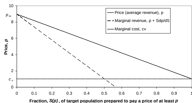
Figure 1. Conventional demand curve.
