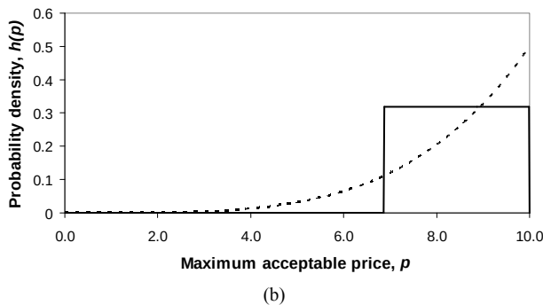
Figure 7. Matching a Rectangular demand density to concave and convex Double Power demand densities when the mode takes the maximum value, p_m . (a) Concave Double Power demand density: b = 0 , c = 0.25 ; (b) Convex Double Power demand density: b = 0 , c = 4.0 .
