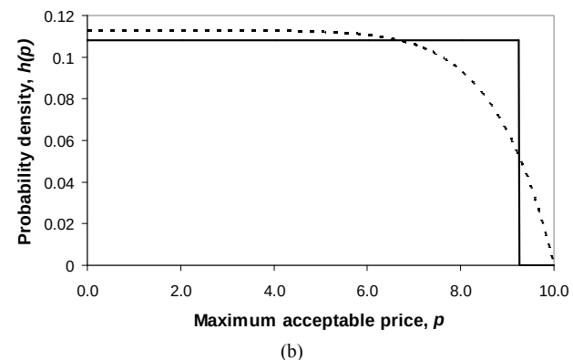
Figure 6. Matching a Rectangular demand density to convex and concave Double Power demand densities when the mode is 0.0. (a) Convex Double Power demand density: c = 0 , d = 0.25 ; (b) Concave Double Power demand density: c = 0 , d = 8.0 .
