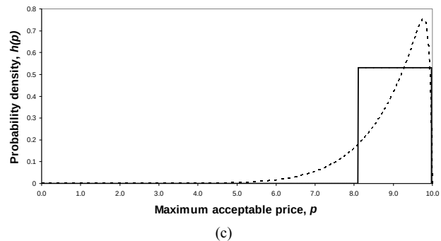
Figure 8. Matching a Rectangular demand density to a Double Power demand density with a strictly interior mode. (a) Double Power demand density. c = 1 , d = 0.5 ; (b) Double Power demand density. c = 2 , d = 4 ; (c) Double Power demand density. c = 8 , d = 128 .
