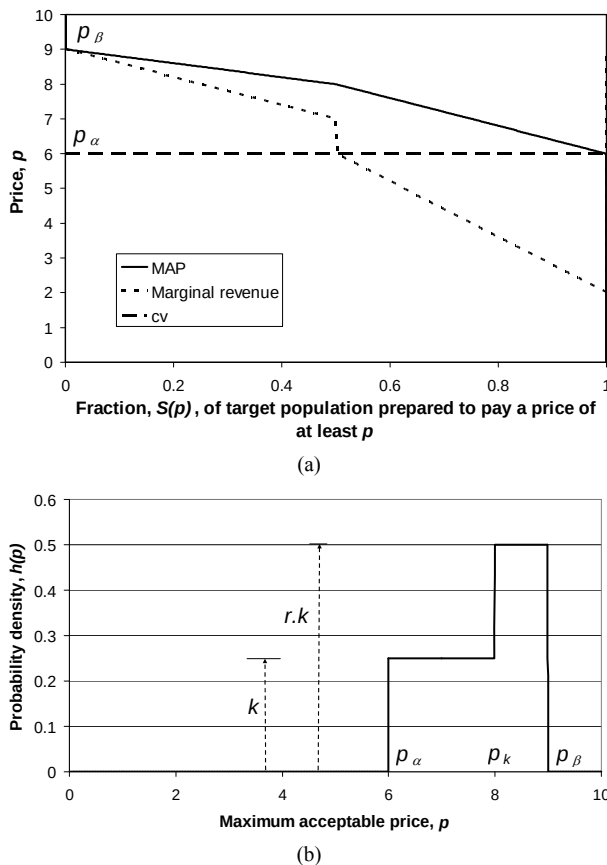
Figure 13. The kinked demand curve and its corresponding demand density. k , r , p_\alpha and p_\beta are defined in Figure 13(b). (a) Demand curve when: r = 2 , p_\alpha = 6 , p_\beta/p_\alpha = 1.5 ; (b) Corresponding demand density.
