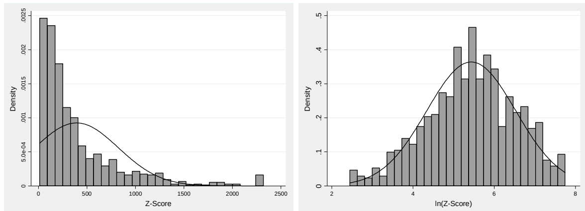
Figure 1 Distribution of Z-Score and Ln(Z-Score)
