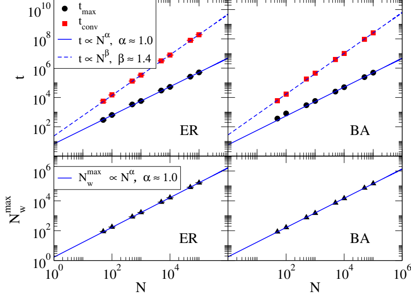
Figure 5: Top: scaling behavior with the system size N for the time of the memory peak ( t_{max} ) and the convergence time ( t_{conv} ) for ER random graphs (left) and BA scale-free networks (right) with average degree \langle k \rangle = 4 . In both cases, the maximal memory is needed after a time proportional to the system size, while the time needed for convergence grows as N^\beta with \beta \simeq 1.4 \pm 0.1 . Bottom: In both networks the necessary memory capacity (i.e. the maximal value N_w^{max} reached by N_w ) scales linearly with the system size.
