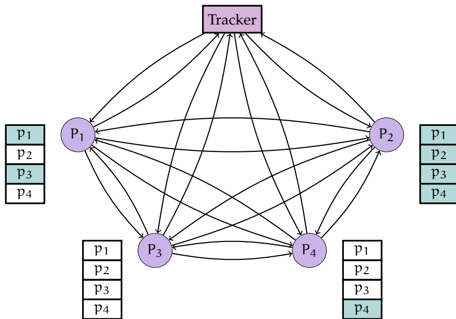
Figure 2.7: Peer P_1 – P_4 represent participating peers and p_1 – p_4 represent a piece of the file. Pieces with a blue background color are pieces which actual peers have and pieces with the a white background are missing pieces. Source: own representation based on [Cho+12].
