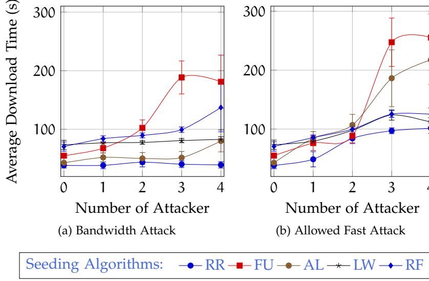
Figure 5.3: File transfer of a 100 MiB file with a piece size of 64 KiB via BitTorrent with a seeder that has 10 Mbps upload limit. (a) A normal bandwidth attack. (b) A bandwidth attack combined with the allowed fast attack. The error bars show 95 % confidence intervals. Source: own representation based on own survey.
