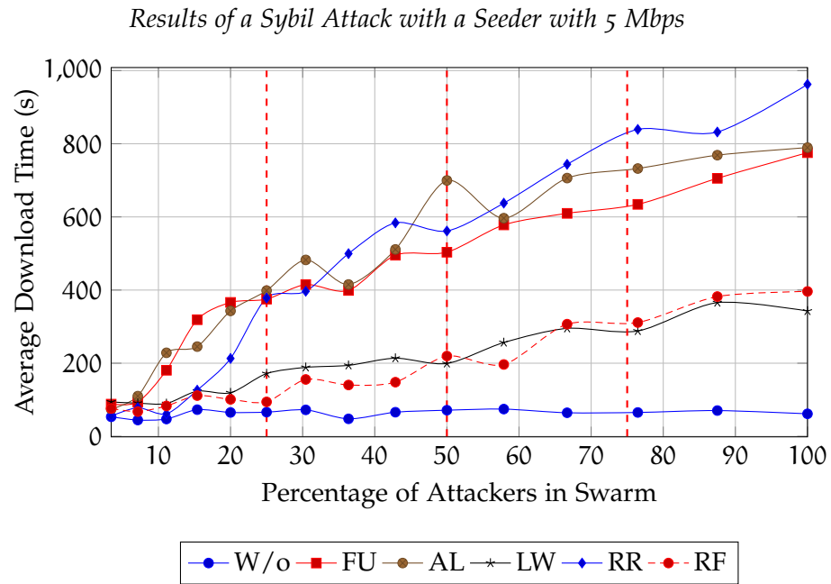
Figure 5.4: File transfer of a 100 MiB file with a piece size of 64 KiB via BitTorrent with a seeder that has a 5 Mbps upload limit. A Sybil attack in which I increased the number of attackers and reduced the number of leechers with every iteration. Source: own representation based on own survey.
