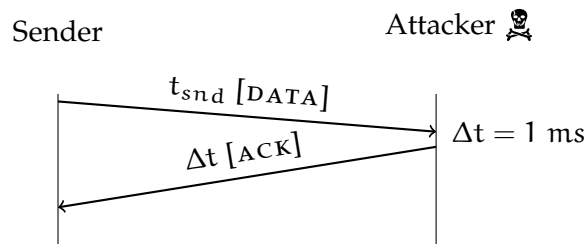
Figure 6.2: One-way delay measurement with a normal receiver and an attacker. Source: own representation.
