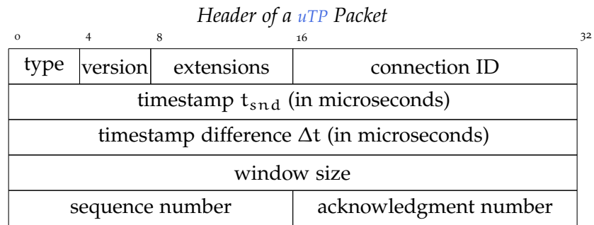
Figure 2.9: Version 1 header of a Micro Transport Protocol (uTP) packet. Source: own representation based on [Nor10].
