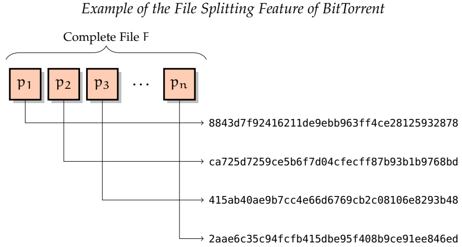
Figure 2.6: A file F which is split into pieces with its Secure Hash Algorithm 1 (SHA-1) hashes. Source: own representation.
