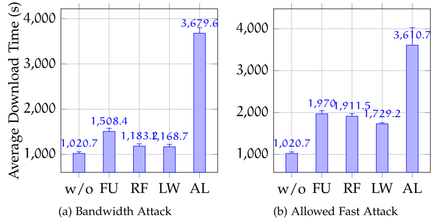
Figure 5.5: File transfer on PlanetLab of a 100 MiB file with a piece size of 64 KiB via BitTorrent. The data was produced with 1 seeder with a 1 Mbps upload limit, 300 leechers with 1 Mbps download limits, and 4 malicious peers. All values are the average values of ten iterations. The error bars show 95 % confidence intervals. Source: own representation based on own survey.
