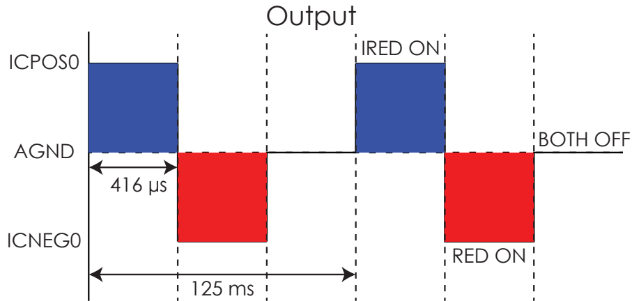
FIGURE 8.8: One of the outputs (ICTRL0) of the dual- 4 channel multiplexer. The infrared LED is first switched on for 416 \mu s, followed by the red LED, and then an off period, where both LEDs are off.
