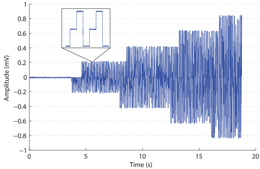
FIGURE 9.7: The accuracy and the sensitivity of measured I_{\text{SENSE0}} to the values set on the front panel.
