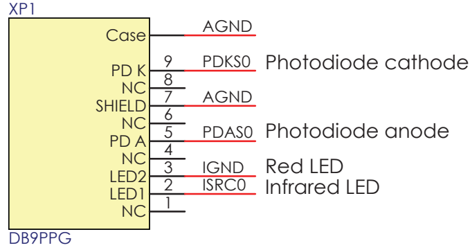
FIGURE 8.16: Pin-out diagram of the DB9 connector.
