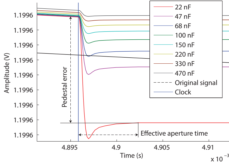
FIGURE 8.37: The sample-to-hold transition of the SHA with various hold capacitors. The offset voltage that appears in the SHA output during this transition is known as pedestal error.
