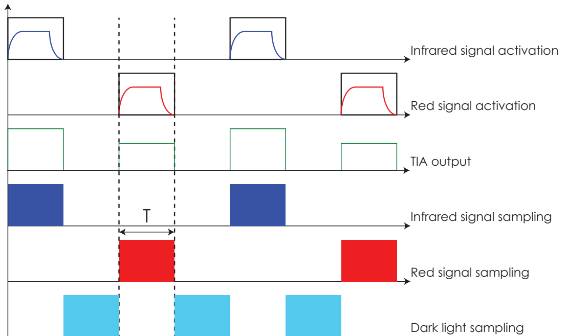
FIGURE 8.20: PPG signal sampling at two different wavelengths using time windowing
