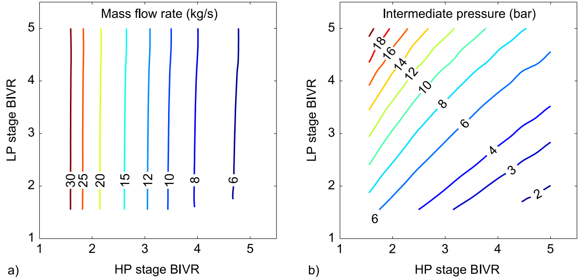
Figure 4: Contour maps showing a) mass flow rate (kg/s) and b) intermediate pressure (bar) of the 2-stage screw expander consisting of 145mm and 408mm machines
