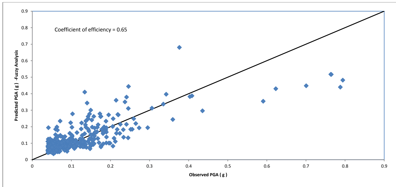
Figure 16. Observed versus Predicted (Fuzzy Analysis) Attenuation Relationships ( g )
