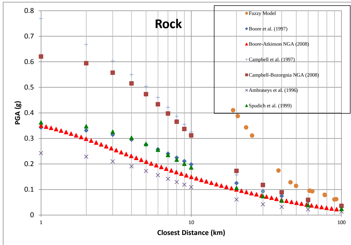
Figure 14. Curves of peak acceleration versus distance for a magnitude 6.5 earthquake at rock sites.
