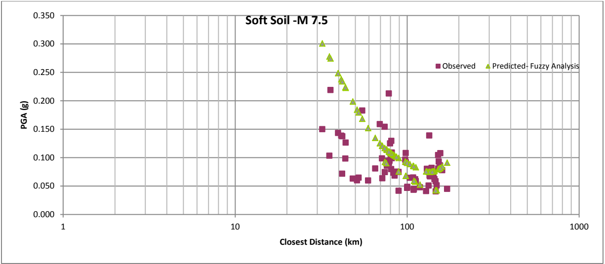
Figure 5. Curves of peak acceleration versus distance for a magnitude 7.5 earthquake at soft soil sites.
