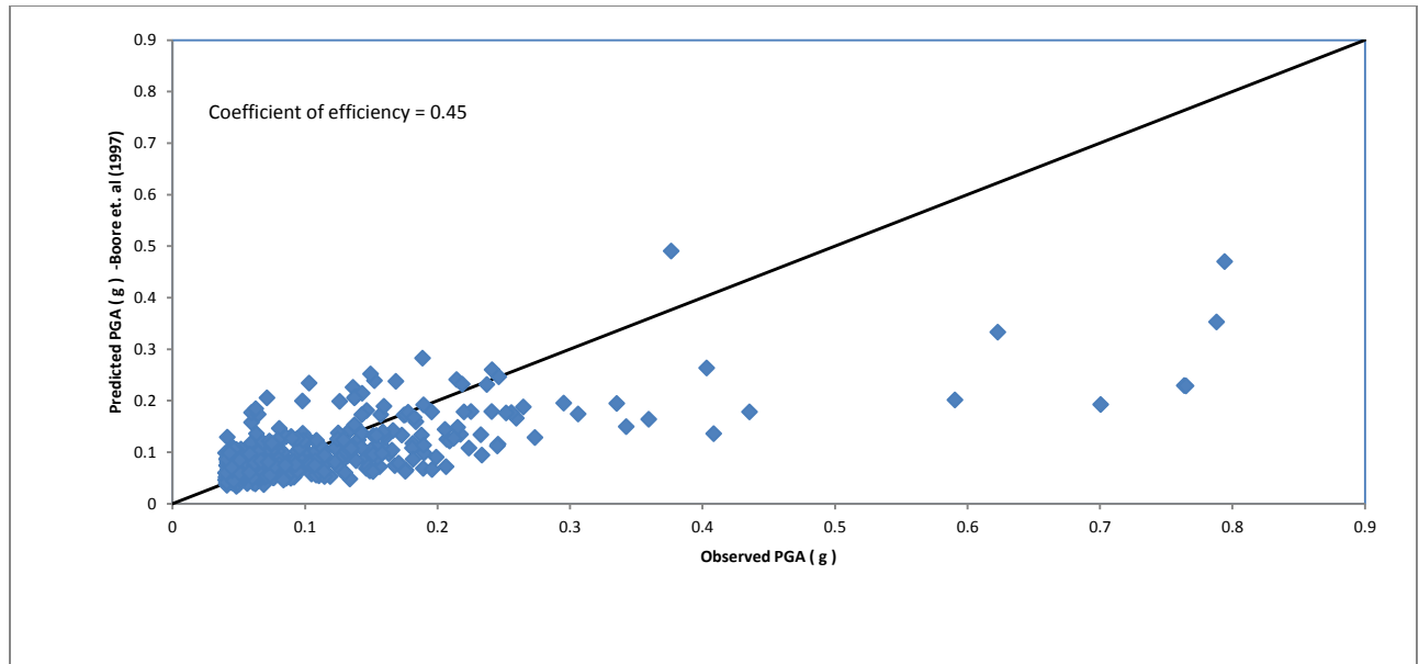
Figure 17. Observed versus Predicted (Boore et. al (1997)) Attenuation Relationships ( g )
