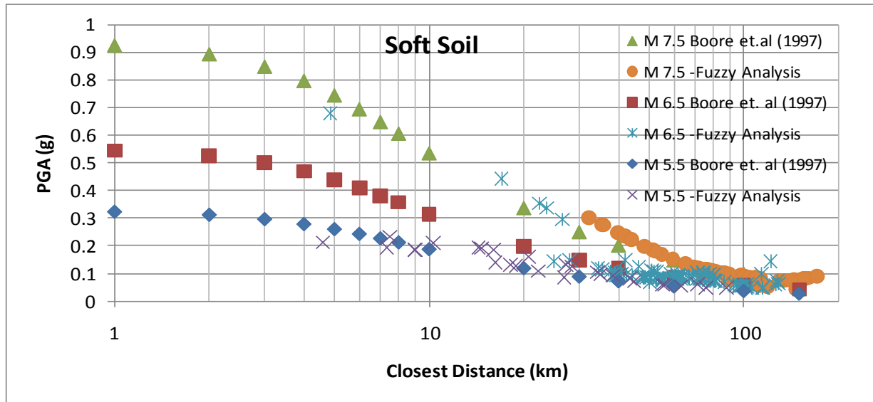
Figure 6. Curves of peak acceleration versus distance for a magnitude 5.5, 6.5 and 7.5 earthquakes at soft soil sites.
