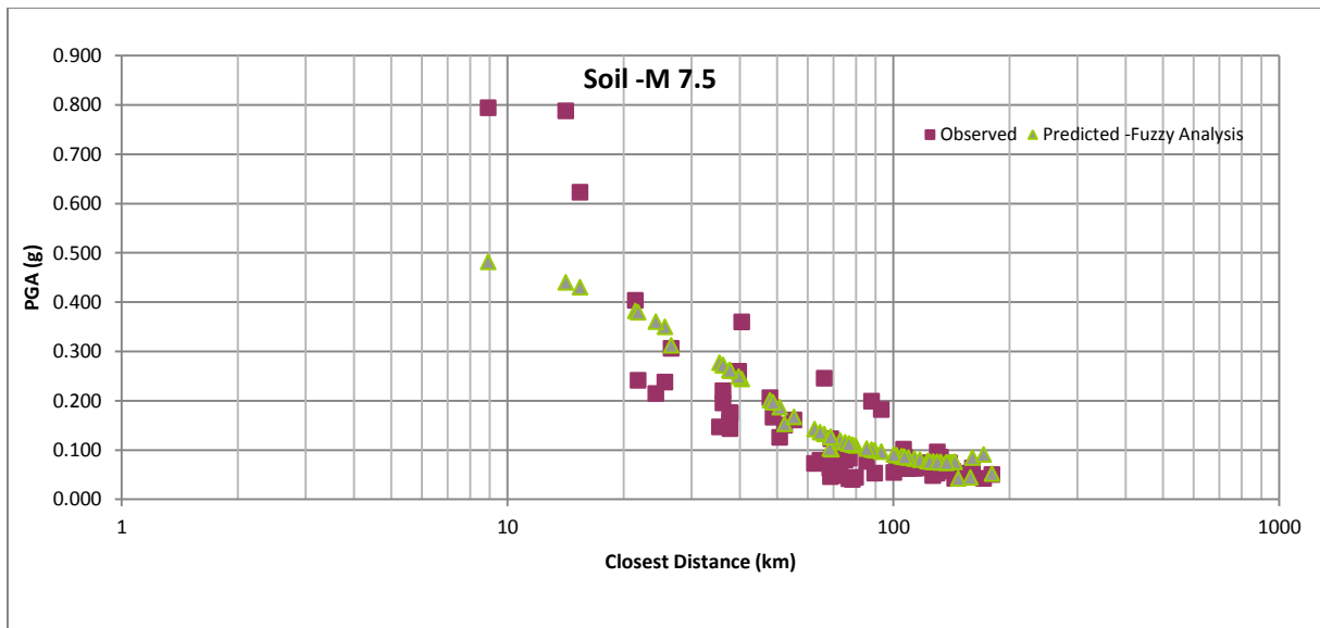
Figure 9. Curves of peak acceleration versus distance for a magnitude 7.5 earthquake at soil sites.
