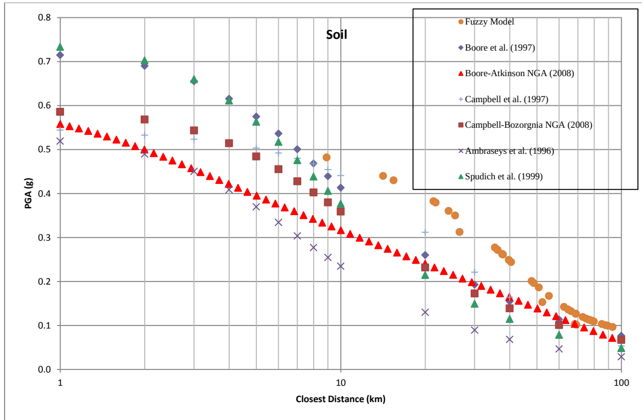
Figure 15. Curves of peak acceleration versus distance for a magnitude 7.5 earthquake at soil sites.
