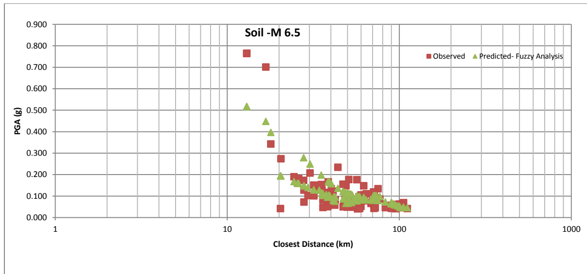
Figure 8. Curves of peak acceleration versus distance for a magnitude 6.5 earthquake at soil sites.
