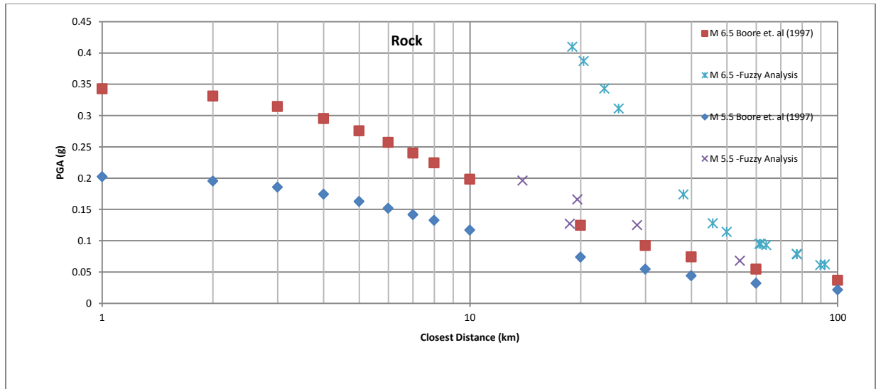
Figure 13. Curves of peak acceleration versus distance for magnitude 5.5 and 6.5 earthquakes at rock sites.
