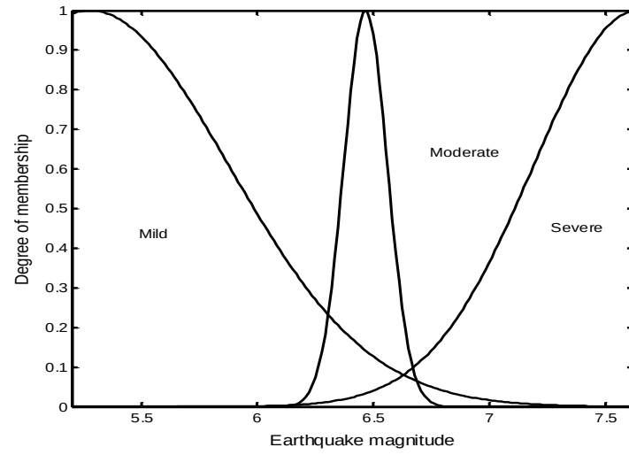
Figure 2. Magnitude Fuzzy Sets
