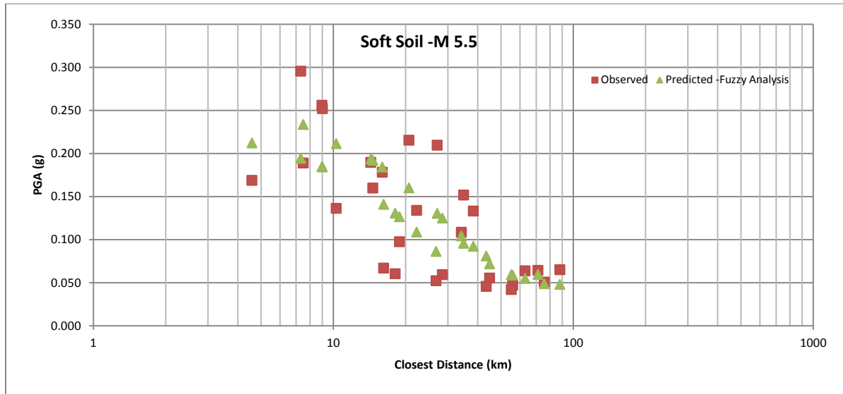
Figure 3. Curves of peak acceleration versus distance for a magnitude 5.5 earthquake at soft soil sites.
