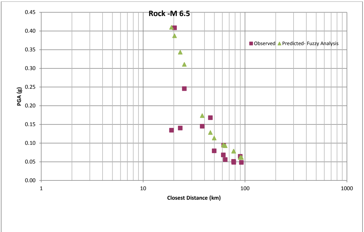
Figure 12. Curves of peak acceleration versus distance for magnitude 6.5 earthquake at rock sites.
