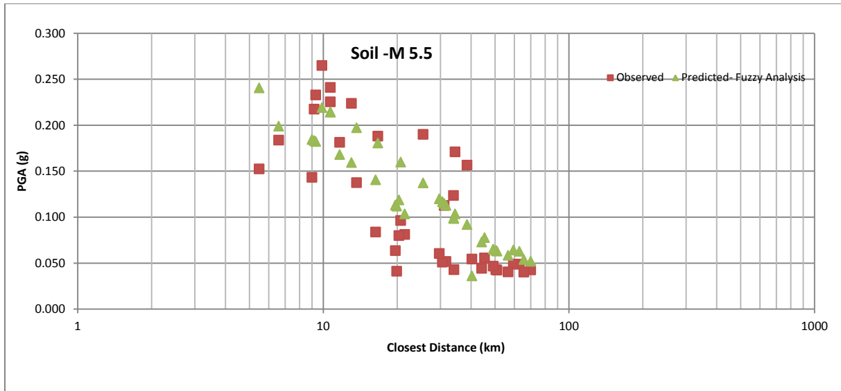
Figure 7. Curves of peak acceleration versus distance for a magnitude 5.5 earthquake at soil sites.
