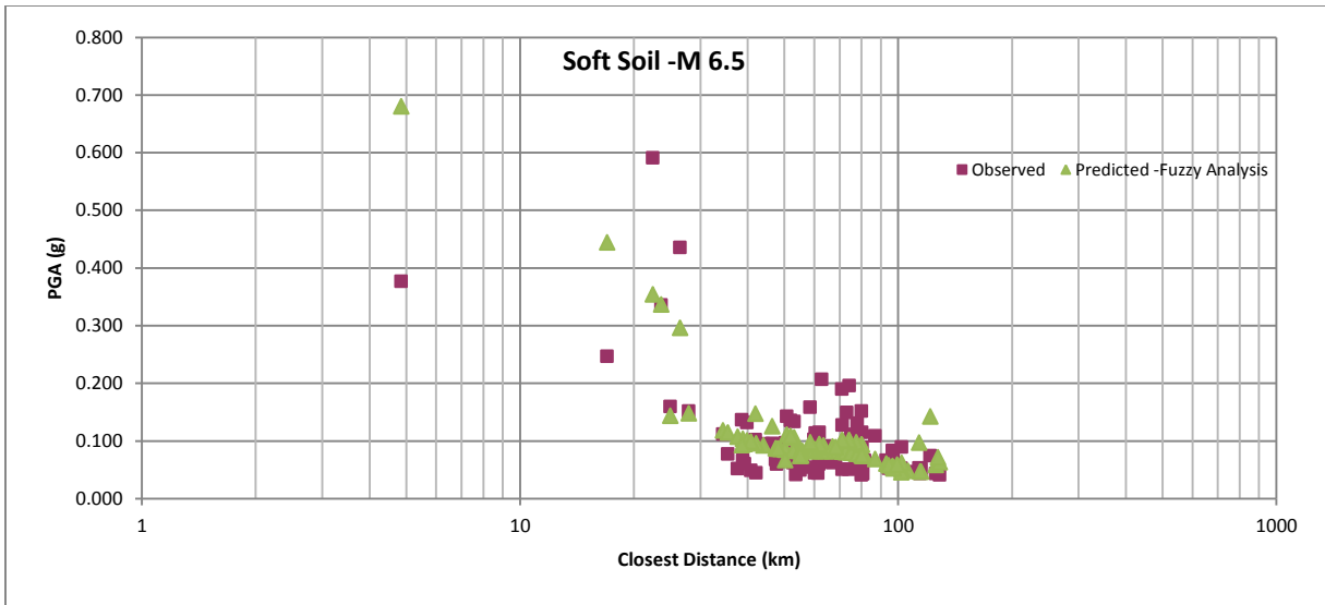
Figure 4. Curves of peak acceleration versus distance for a magnitude 6.5 earthquake at soft soil sites.
