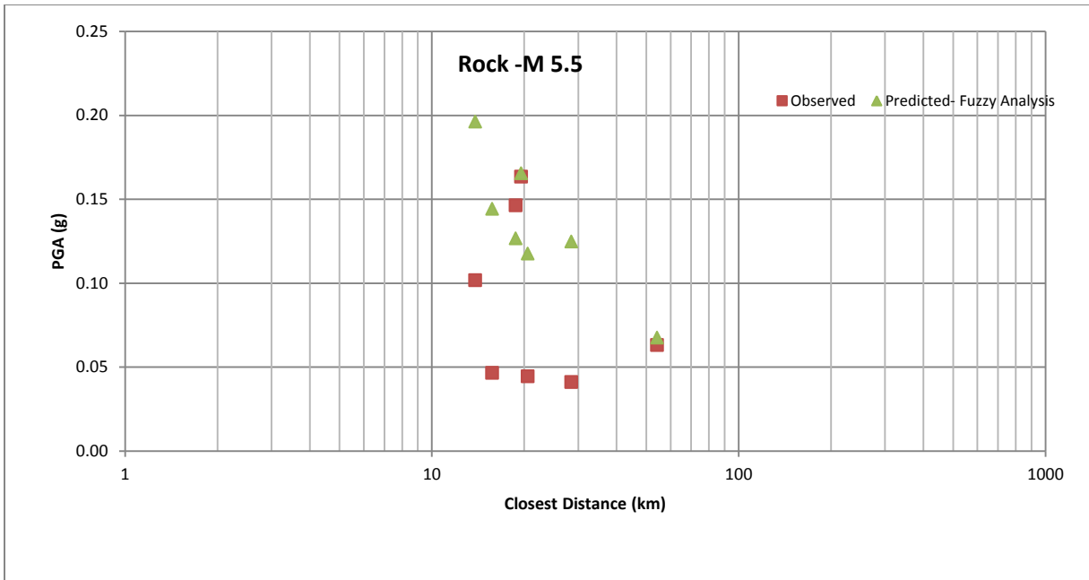
Figure 11. Curves of peak acceleration versus distance for a magnitude 5.5 earthquake at rock sites.
