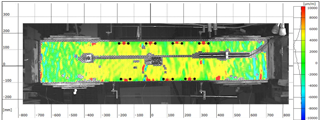
Fig. 5. Full strain field in the direction of applied load of a specimen at a specific load level
