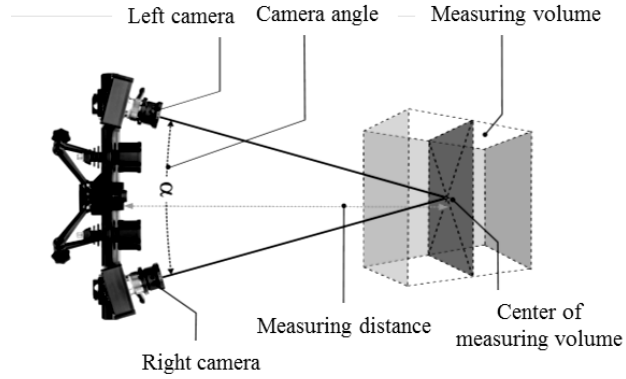
Fig.4. ARAMIS 3D sensor setup
