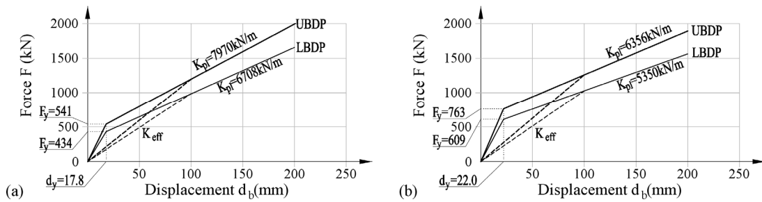
Figure 7: Bounding Design Properties of Lead-Rubber Bearings (a) LRB 1200×1200/231-200 (b) LRB 1200×1200/286-250
