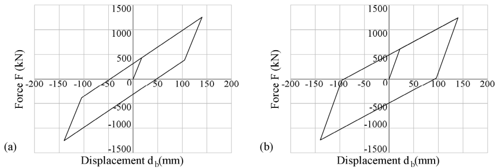
Figure 12: Simplified bilinear hysteresis loops of LRBs at the design displacement (a) LRB 1200×1200/231-200 (b) LRB 1200×1200/286-250
