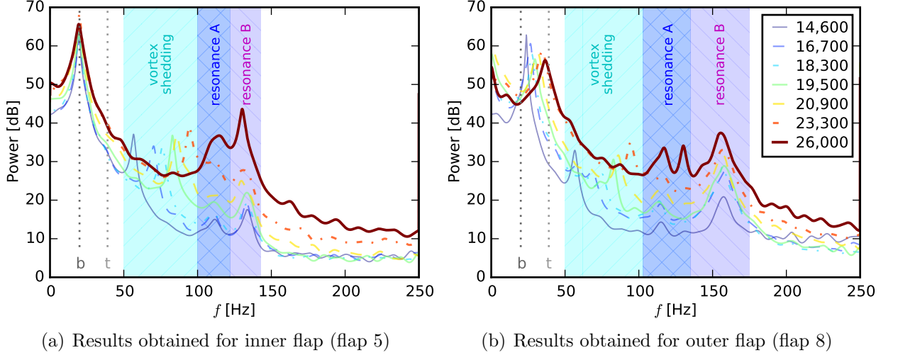
Figure 12: Spectra obtained for the movement of one inner flap and one outer flap using a Burg algorithm [33] for different Reynolds numbers (dotted gray lines represent the eigenfrequencies of the first bending mode, b , and the first torsional mode, t , of the single flaps)
