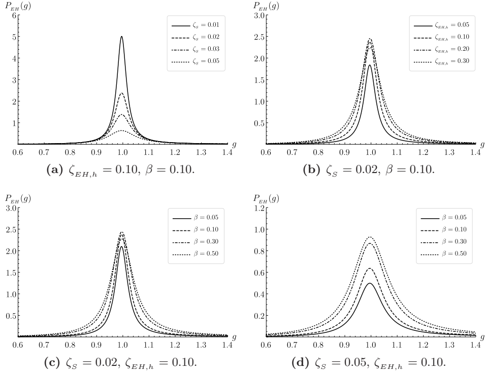
Figure 3. Harvested energy P_{EH}(g) with \mu = 0.01, \zeta_{EH,p} = 0.01 .
