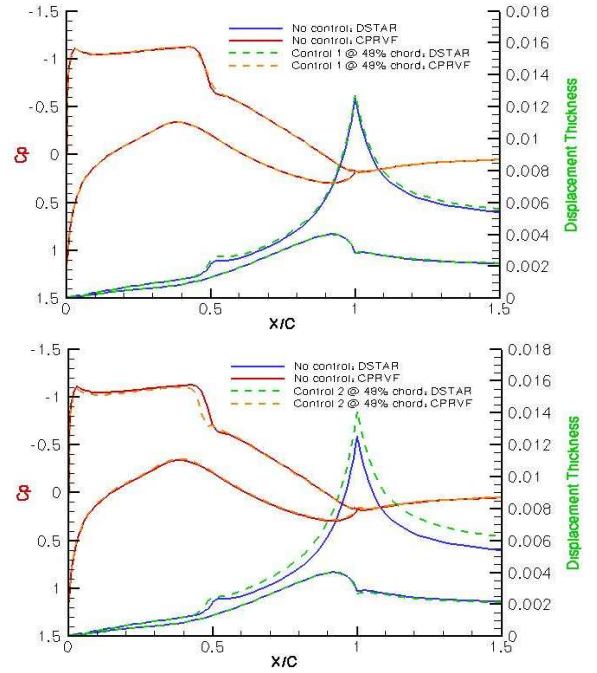
Fig. 12. Surface pressure and displacement thickness distributions on the RAE 2822 aerofoil at Mach 0.725, Reynolds number 6.5 million, incidence 2.5^\circ with and without a viscous ramp at 48% chord. In the upper figure the control is applied only to displacement thickness \delta^* ; in the lower figure, to both \delta^* and \theta .
