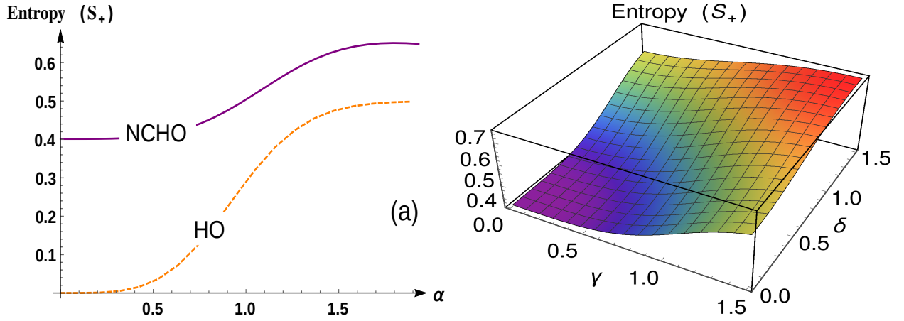
Figure 4: Linear entropy for even cat states (a) of ordinary harmonic oscillator (orange, dashed) versus noncommutative harmonic oscillator (purple, solid), (b) of noncommutative harmonic oscillator in the complex plane of \alpha , with \alpha = \gamma + i\delta and \tau = 2 .
