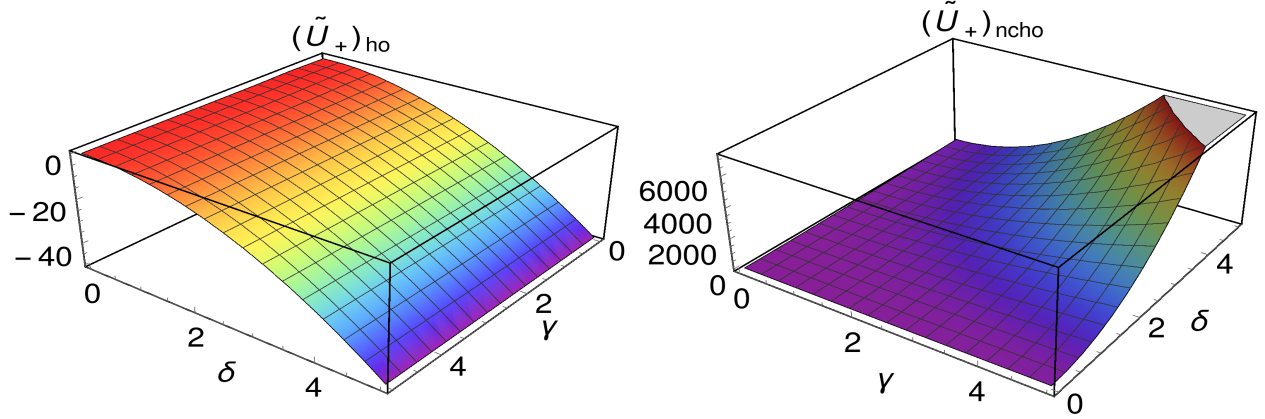
Figure 2: Expansion of quadrature z for ordinary harmonic oscillator (left panel) versus squeezing of quadrature Z for noncommutative harmonic oscillator for \tau = 5 (right panel) in the complex plane of \alpha , with \alpha = \gamma + i\delta .
