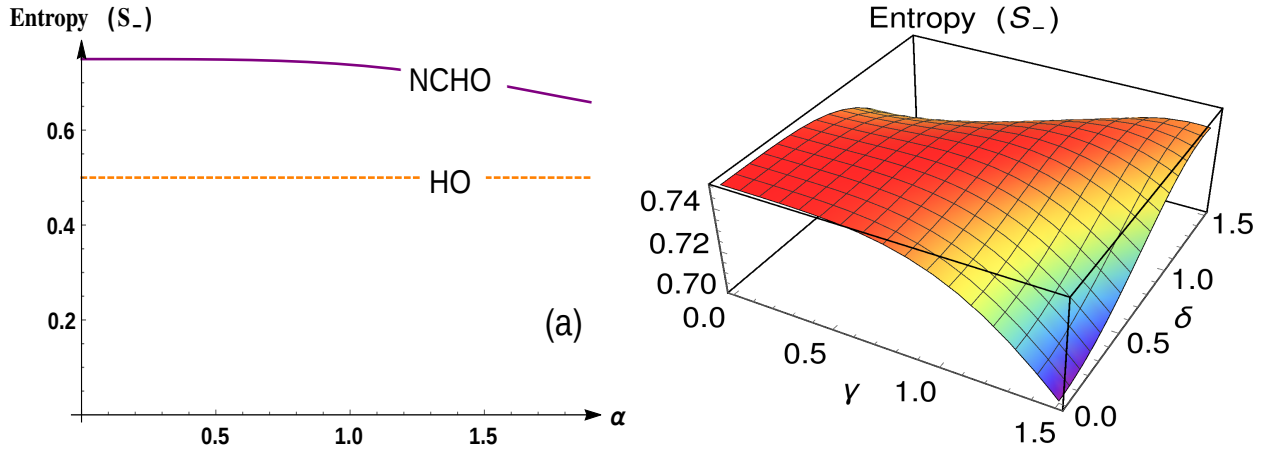
Figure 7: Linear entropy for odd cat states (a) of ordinary harmonic oscillator (orange, dashed) versus noncommutative harmonic oscillator (purple, solid), (b) of noncommutative harmonic oscillator in the complex plane of \alpha , with \alpha = \gamma + i\delta and \tau = 2 .
