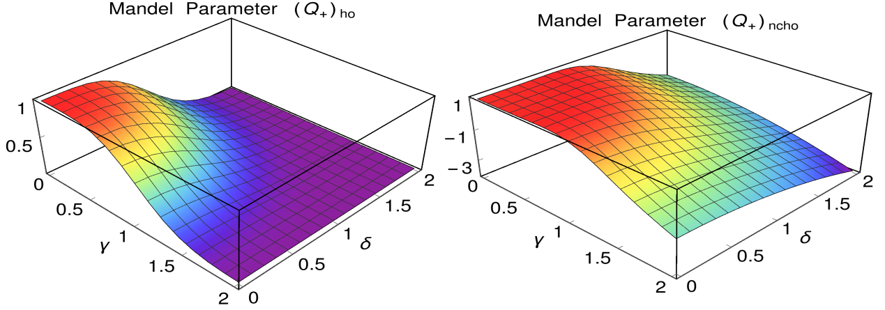
Figure 3: Mandel parameter of even cat states in complex plane of \alpha , with \alpha = \gamma + i\delta for harmonic oscillator (left panel), for noncommutative harmonic oscillator for \tau = 1 (right panel).
