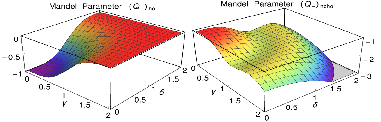
Figure 6: Mandel parameter of odd cat states in complex plane of \alpha , with \alpha = \gamma + i\delta for harmonic oscillator (left panel), for noncommutative harmonic oscillator for \tau = 1 (right panel).
