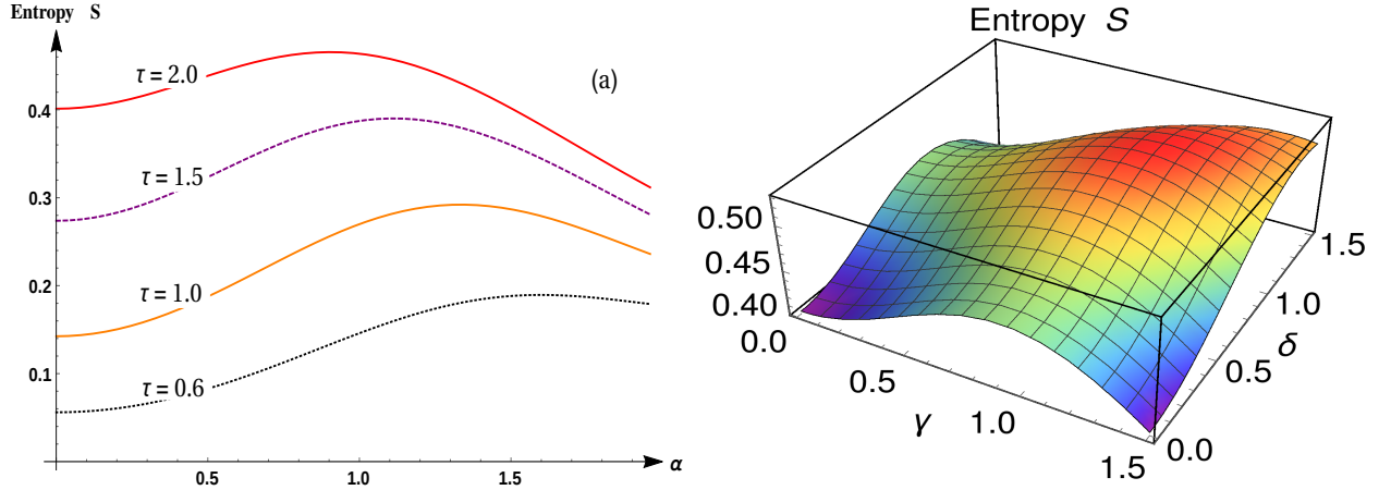
Figure 1: Linear entropy of noncommutative coherent states (a) for different values of \tau , (b) in the complex plane of \alpha , with \alpha = \gamma + i\delta and \tau = 2 .
