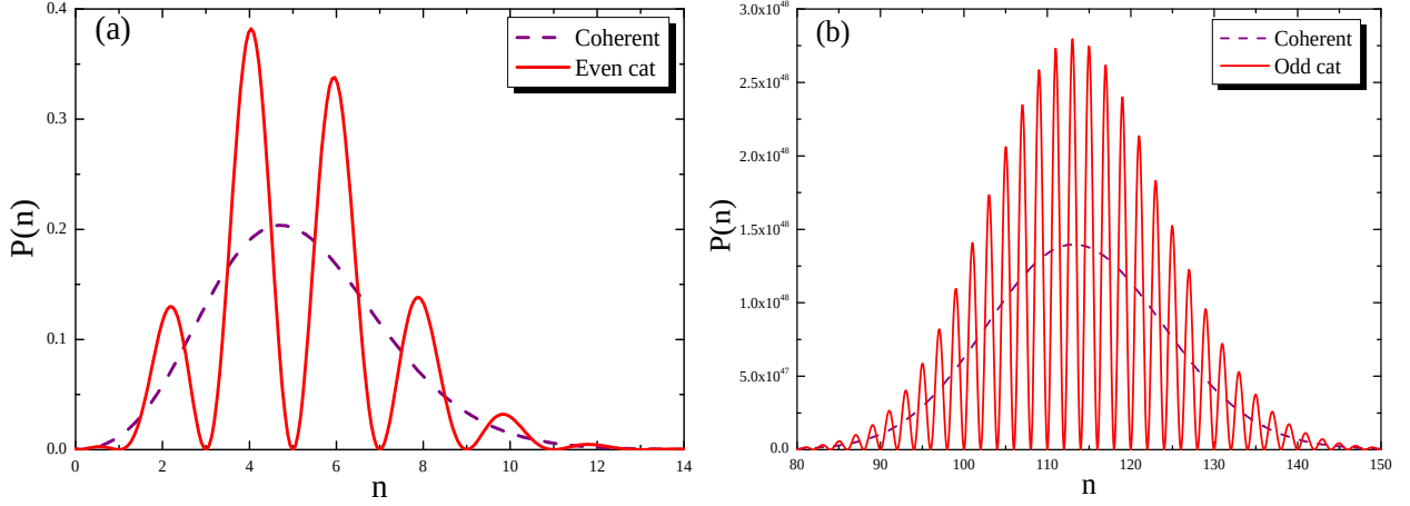
Figure 5: Photon distribution functions of coherent states (purple, dashed) versus (a) even cat states (red, solid) for \alpha = 1.2 + 1.5i , (b) odd cat states (red, solid) for \alpha = 1.2 + 10.5i in noncommutative space for \tau = 10 .
