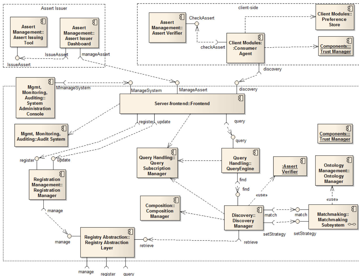
Fig. 1. Architecture Overview
