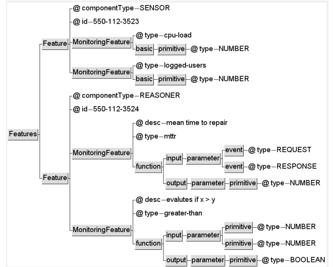
Figure 3: Component Monitoring Features as XML Elements
