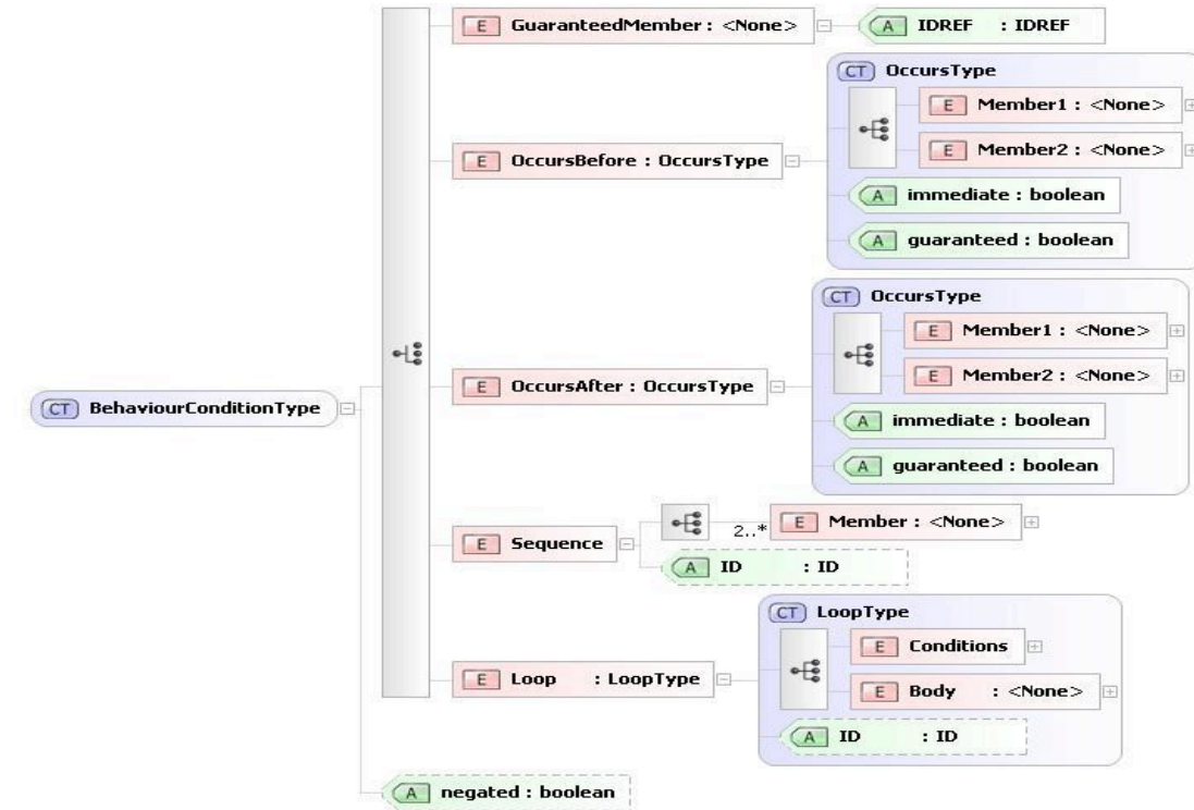
Fig. 6 XML Schema for behavioral criteria
